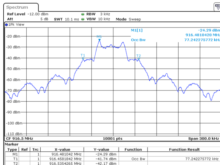
Plot 7.3.2 Occupied bandwidth test result 99%
