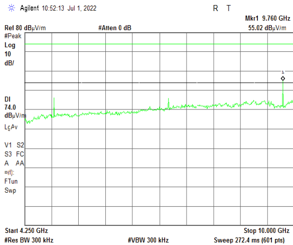
Plot 7.3.21 Radiated emission measurements from 4250 to 10000 MHz at the high carrier frequency
