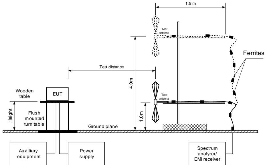
Figure 7.3.2 Setup for spurious emission field strength measurements from 30 to 1000 MHz
