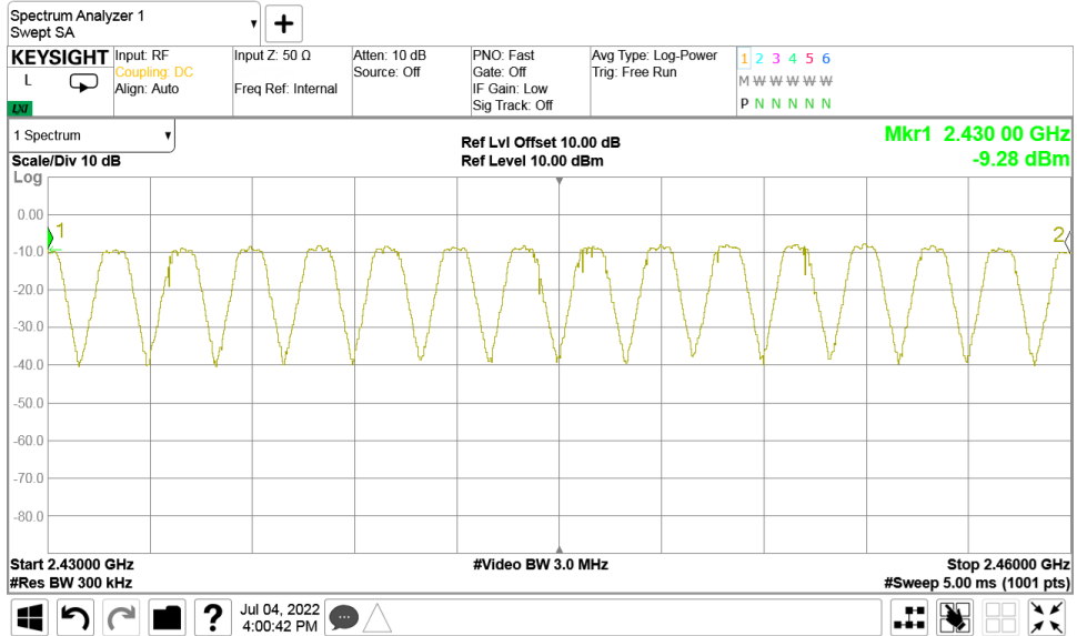
Plot 7.3.2 Number of hopping frequencies (continuation)
