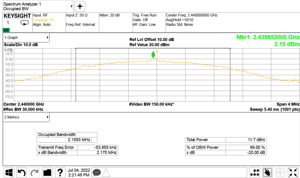
Plot 7.1.2 The 20 dB bandwidth test result at mid frequency at Data Rate = LE_2M_prbs9
