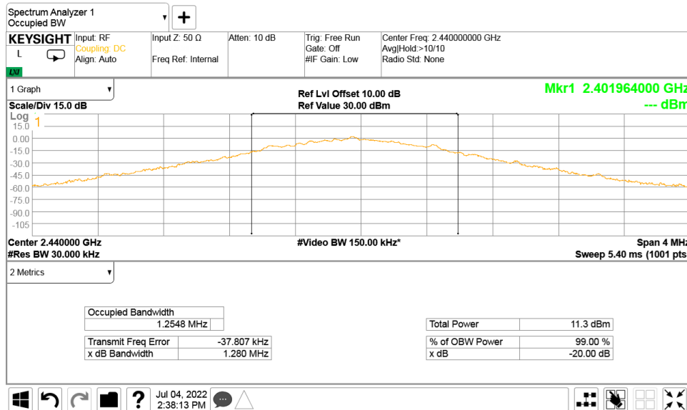
Plot 7.1.11 The 20 dB bandwidth test result at mid frequency at Data Rate = LE_1M_prbs9
