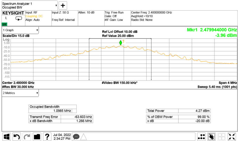
Plot 7.1.18 The 20 dB bandwidth test result at high frequency at Data Rate = LE_1M_00001111
