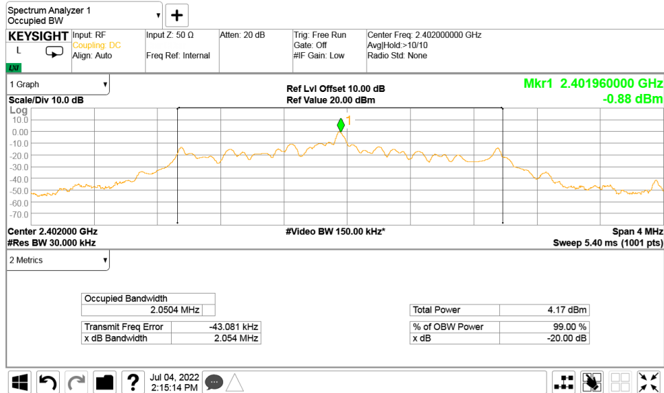
Plot 7.1.4 The 20 dB bandwidth test result at low frequency at Data Rate = LE_2M_1010
