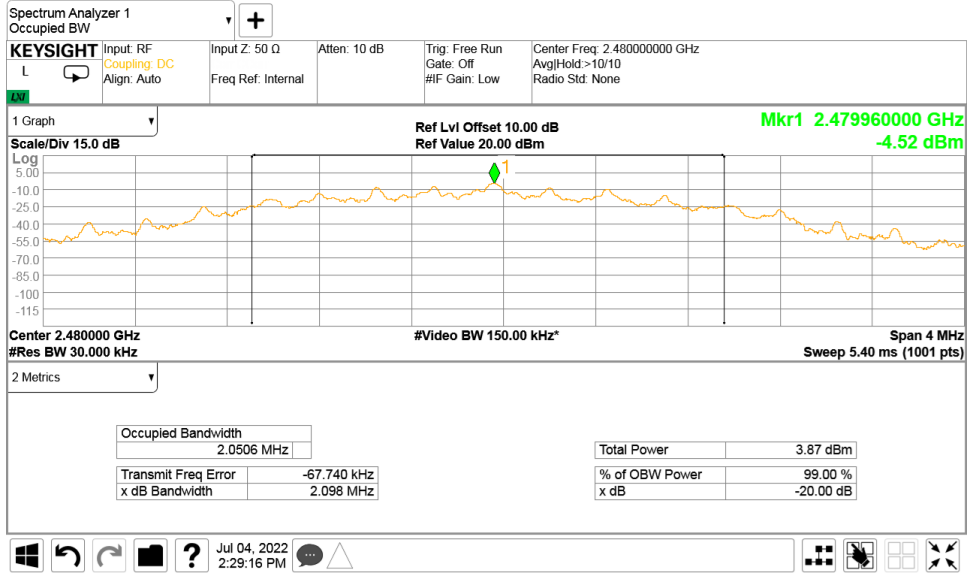
Plot 7.1.9 The 20 dB bandwidth test result at high frequency at Data Rate = LE_2M_00001111
