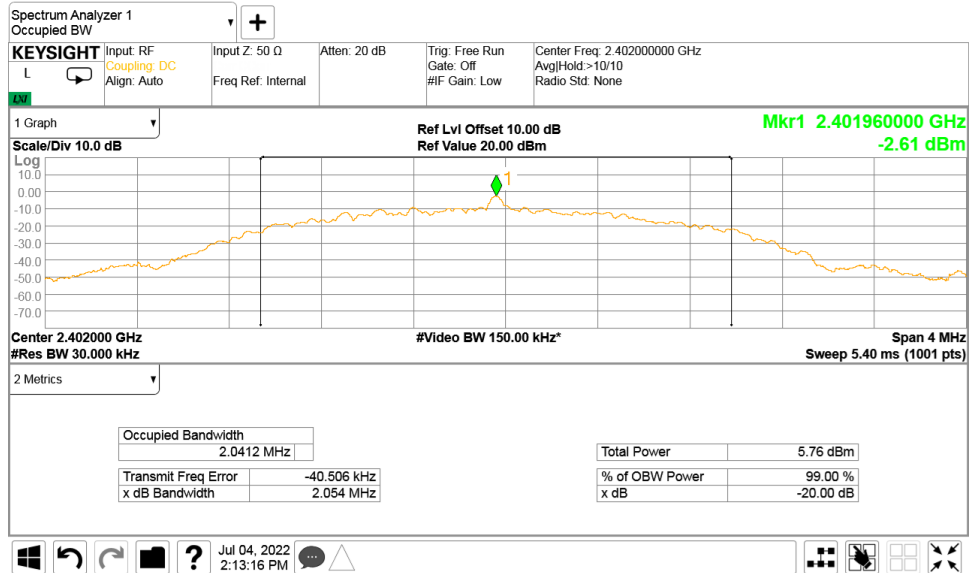
Plot 7.1.1 The 20 dB bandwidth test result at low frequency at Data Rate = LE_2M_prbs9
