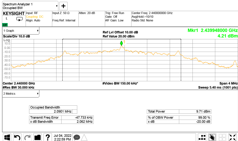
Plot 7.1.5 The 20 dB bandwidth test result at mid frequency at Data Rate = LE_2M_1010
