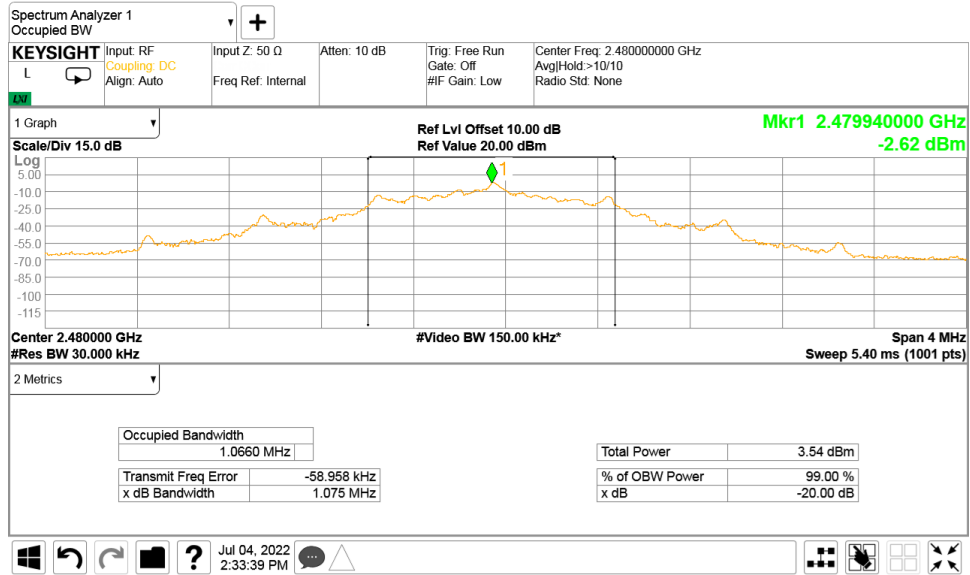
Plot 7.1.15 The 20 dB bandwidth test result at high frequency at Data Rate = LE_1M_1010
