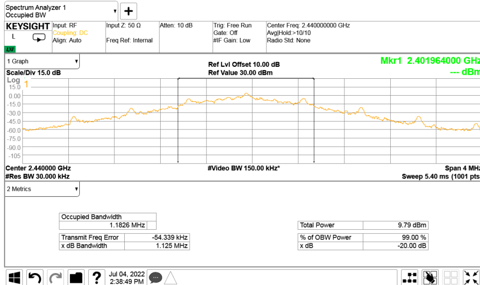
Plot 7.1.14 The 20 dB bandwidth test result at mid frequency at Data Rate = LE_1M_1010
