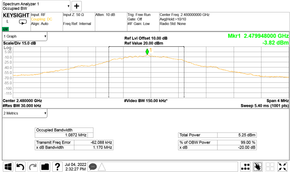
Plot 7.1.12 The 20 dB bandwidth test result at high frequency at Data Rate = LE_1M_prbs9
