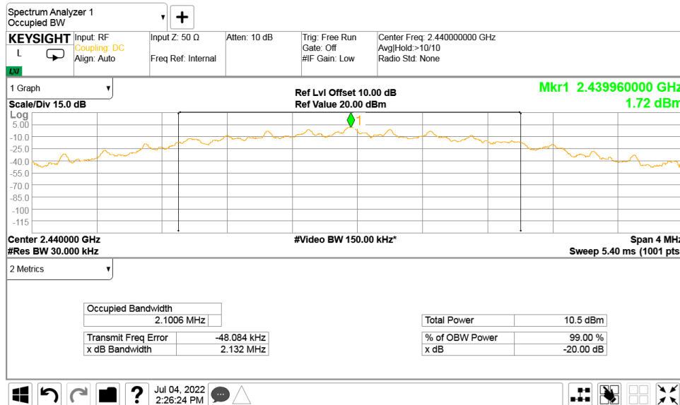
Plot 7.1.8 The 20 dB bandwidth test result at mid frequency at Data Rate = LE_2M_00001111
