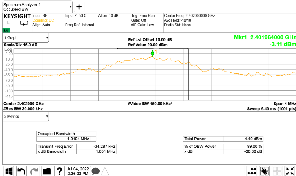
Plot 7.1.16 The 20 dB bandwidth test result at low frequency at Data Rate = LE_1M_00001111
