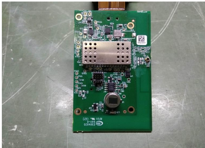
Photograph 7.5.1 Antenna assembly
