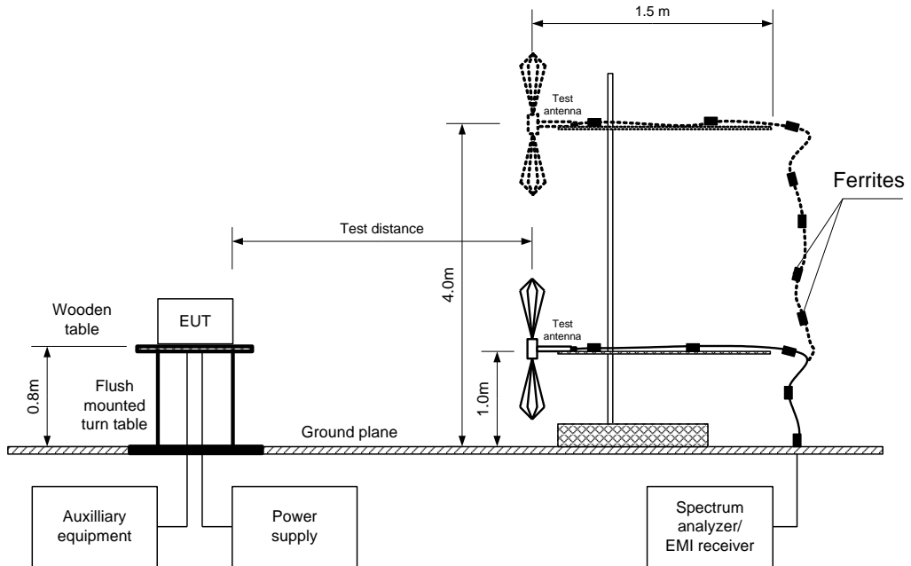
Figure 7.2.2 Setup for spurious emission field strength measurements in 30 -1000 MHz
