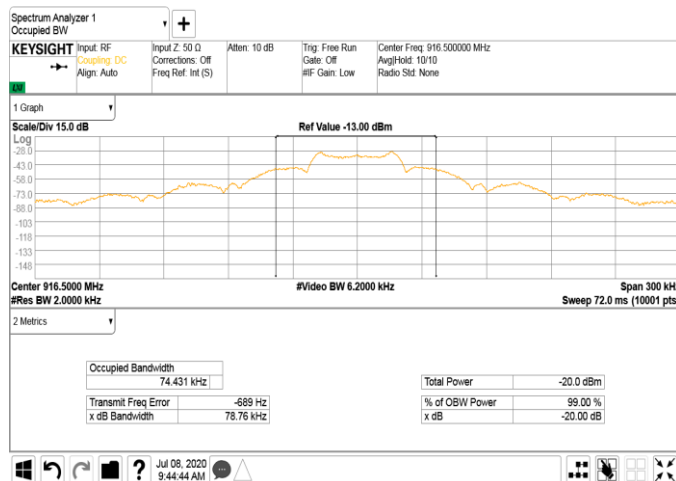
Plot 7.3.1 Occupied bandwidth test results
