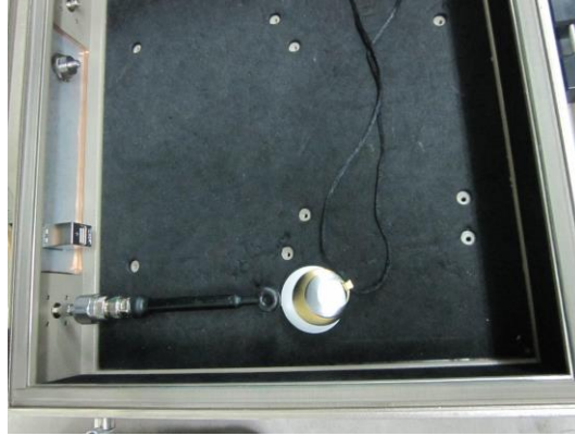
Photograph 1 Setup for OBW measurements
