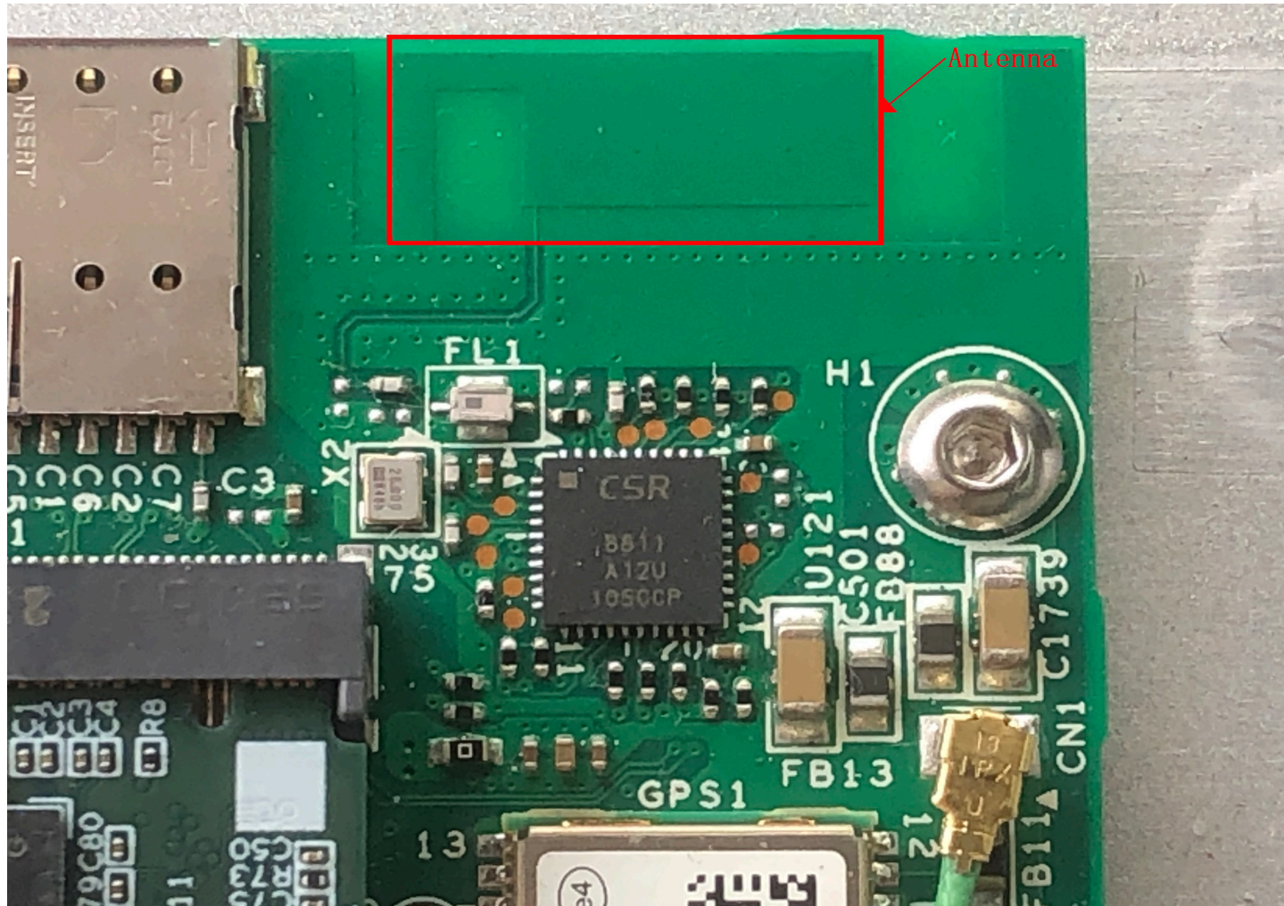
2.4GHz BT Antenna
