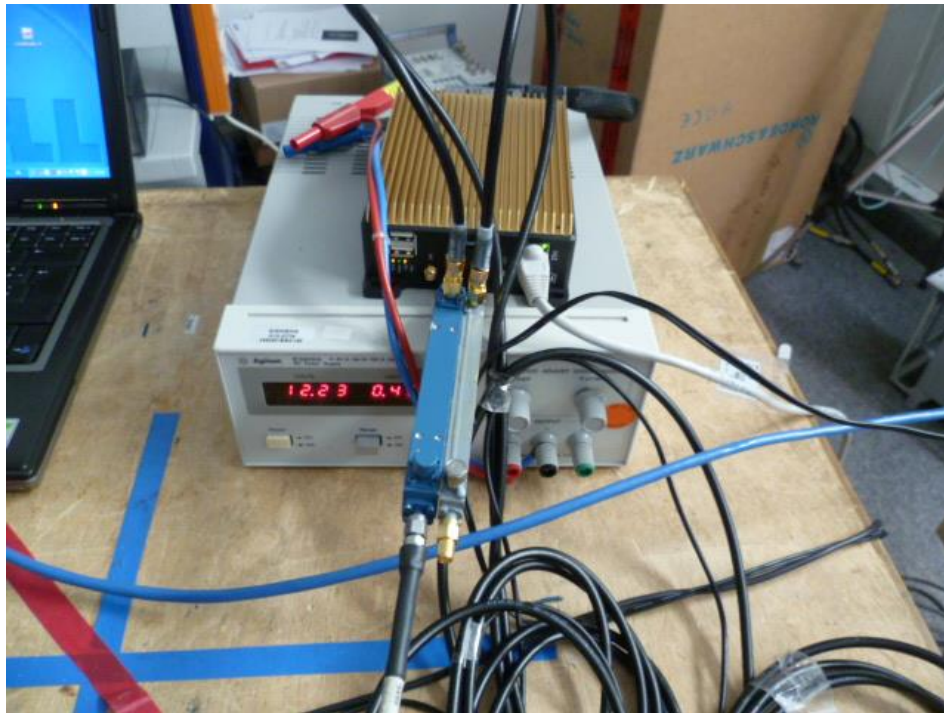
Figure 3: μCROS SL Close View Conducted Sample for WLAN Testing
