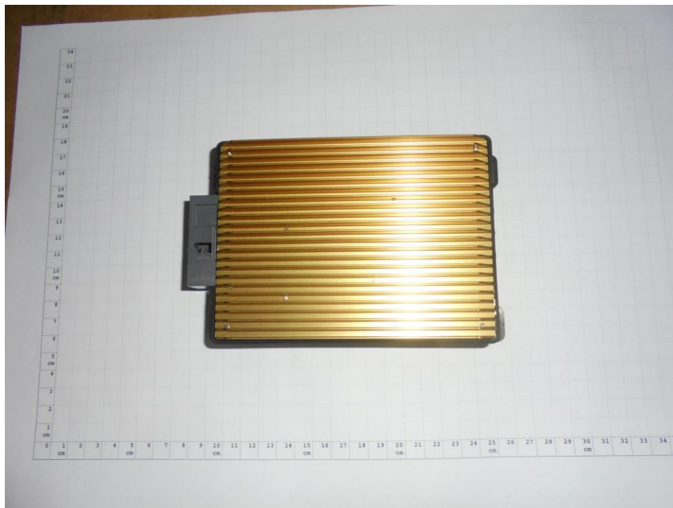
Figure 1: EUT top side view
