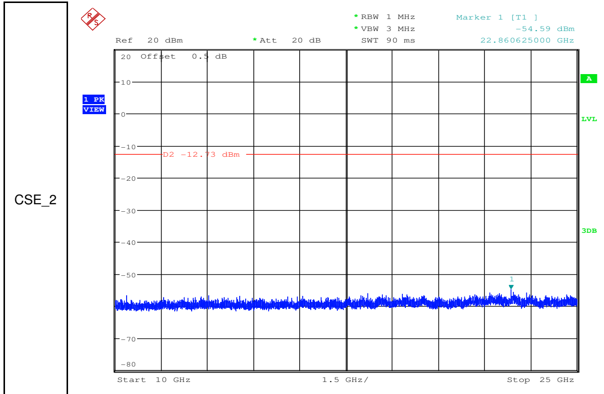
RF Conducted Spurious Emissions_11B_2437_Ant1
