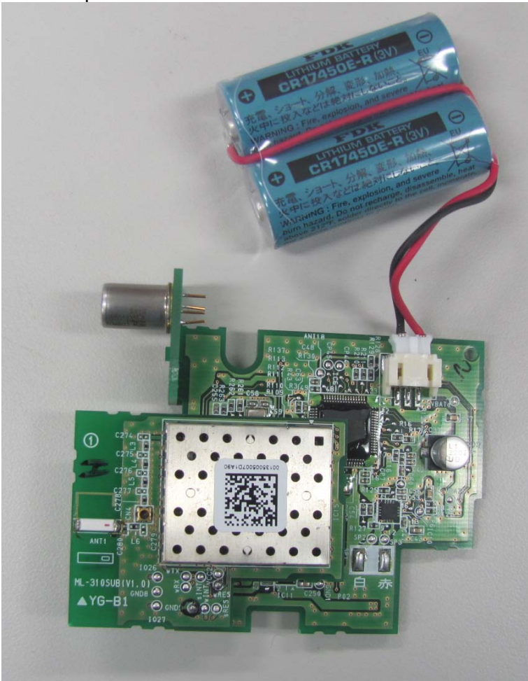
Assembly with Battery; Speaker wire removed to show more detail
