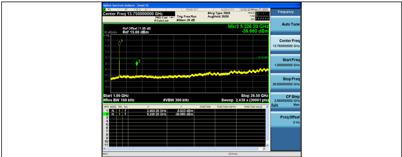
11G-Ant1-2412-0~Reference--6.49
