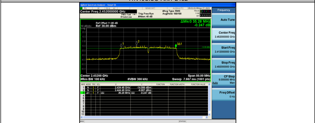
11N40SISO-Ant1-2452
