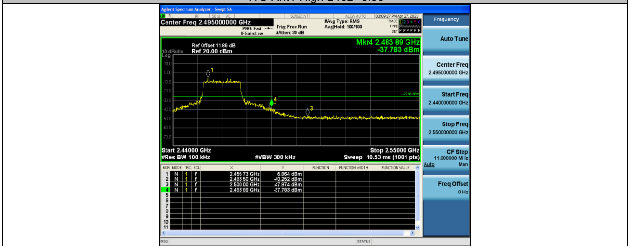
11N20SISO-Ant1-Low-2412--6.68
