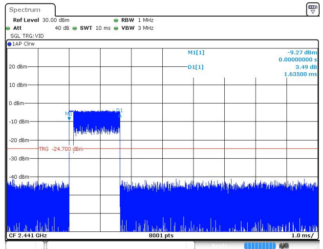
Channel 39 / 2441 MHz - 2DH3
