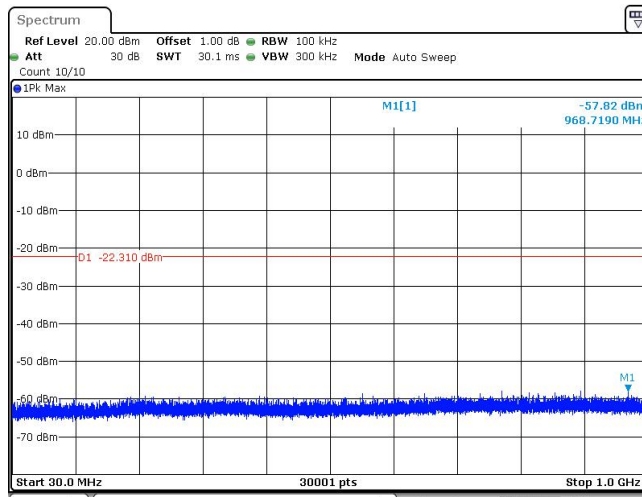
30MHz~1GHz
