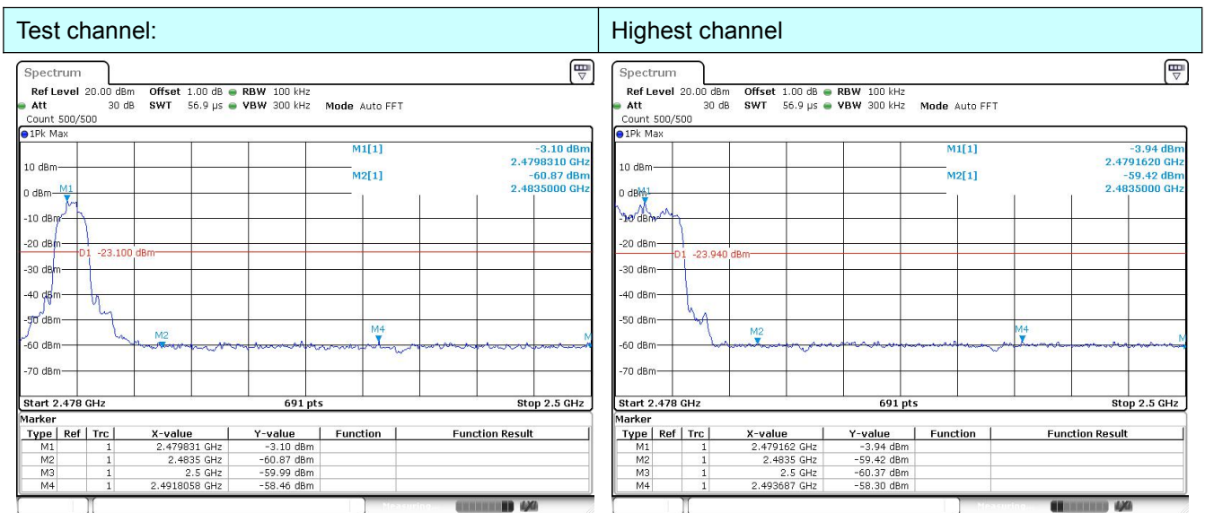
No-hopping mode
