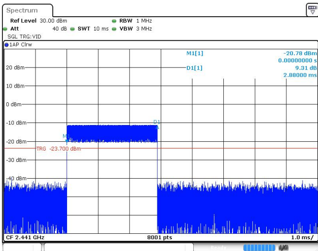
Channel 39 / 2441 MHz - DH5
