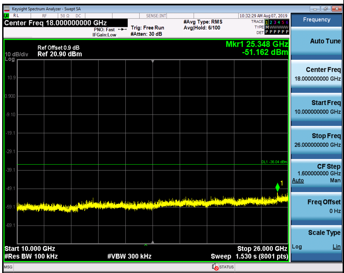
RF Conducted Spurious Emissions_11N40SISO_2442_Ant1
