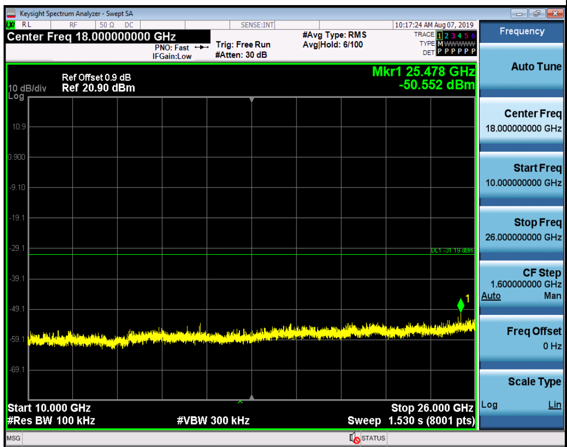
RF Conducted Spurious Emissions_11G_2442_Ant1
