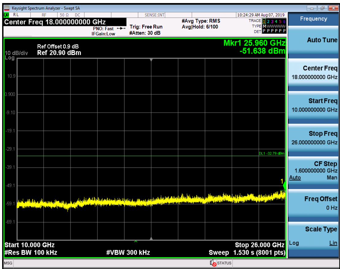
RF Conducted Spurious Emissions_11N20SISO_2442_Ant1
