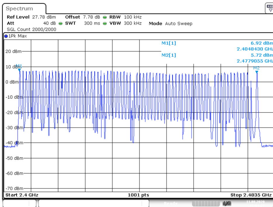
Hopping No. NVNT user 2441MHz
