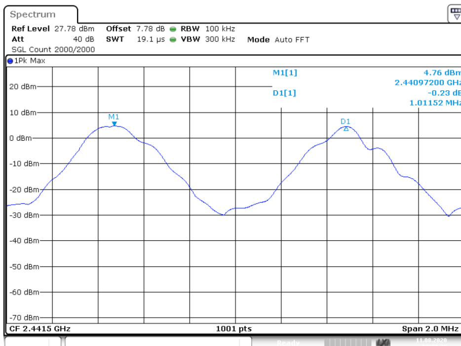
CFS NVNT user 2441MHz
