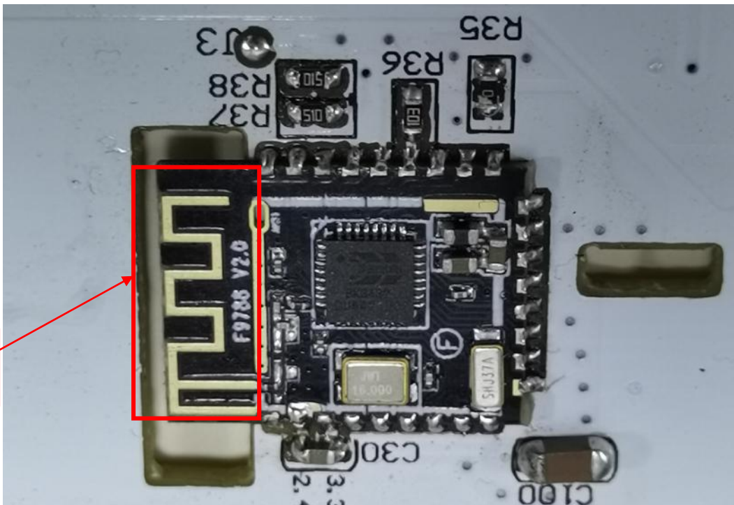
BT Antenna
