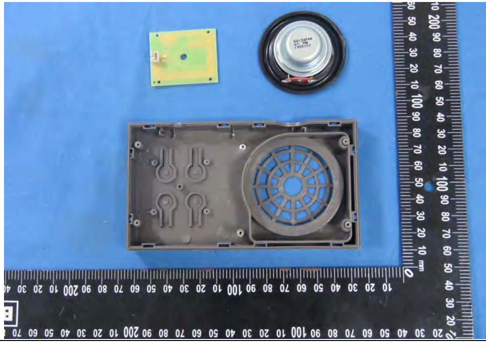
EUT Photo (28)
