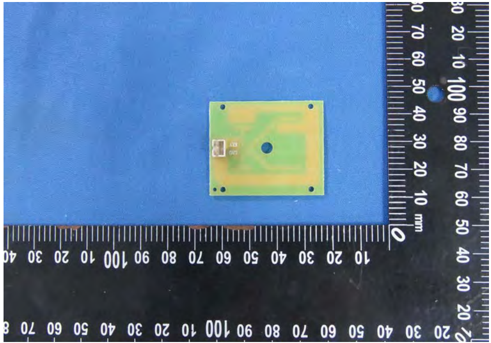
EUT Photo (32)
