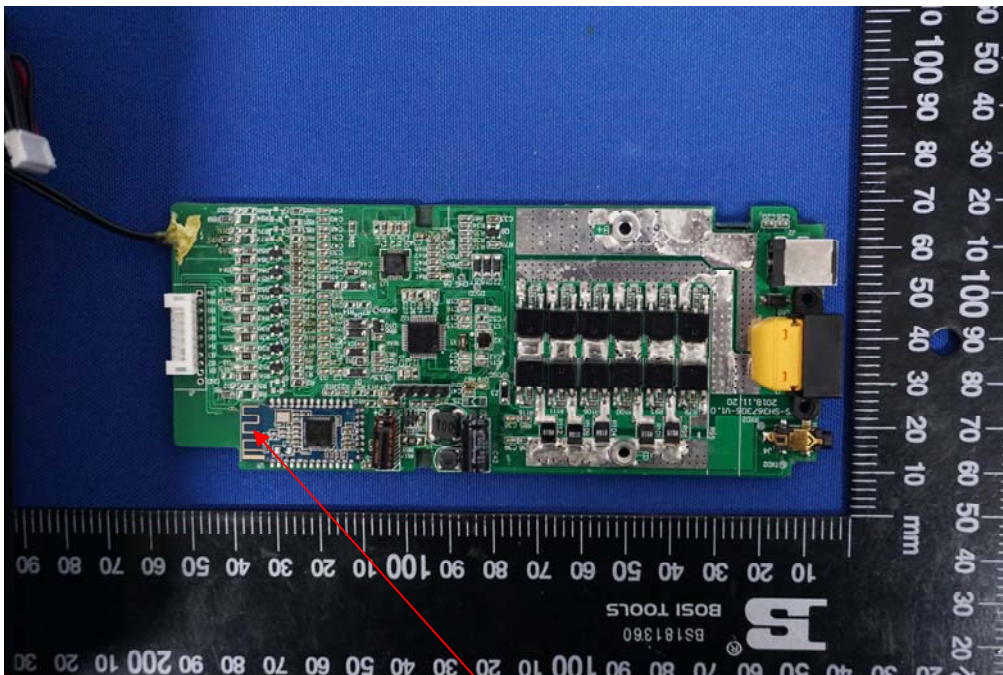
BT Antenna
