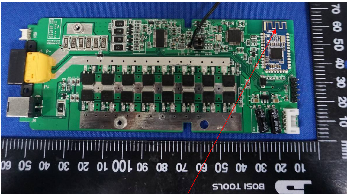
BT Antenna
