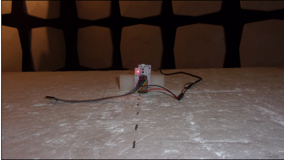
Figure 6: Radiated Emissions – YPOS
