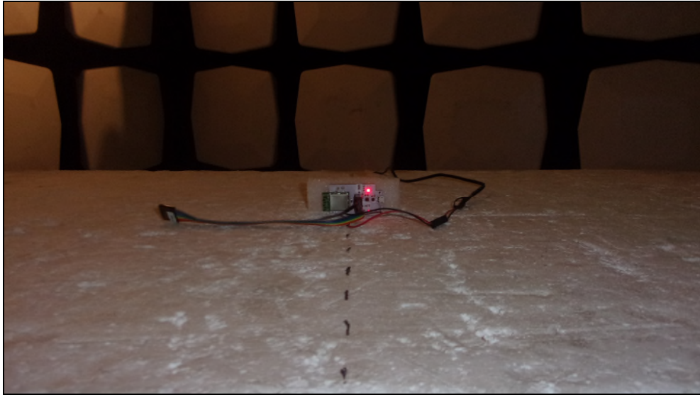
Figure 5: Radiated Emissions – XPOS
