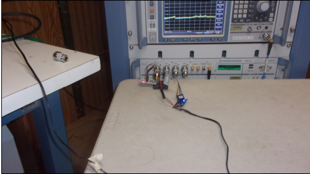
Figure 8: Conducted RF Measurements
