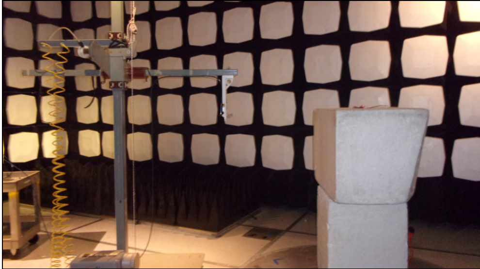
Figure 4: Radiated Emissions – 18GHz – 25GHz
