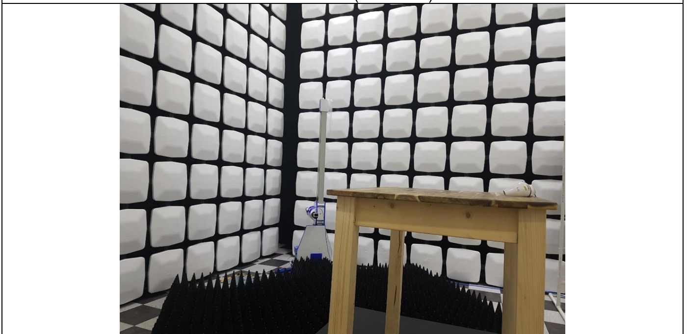
Radiated Test (Above 1G)
