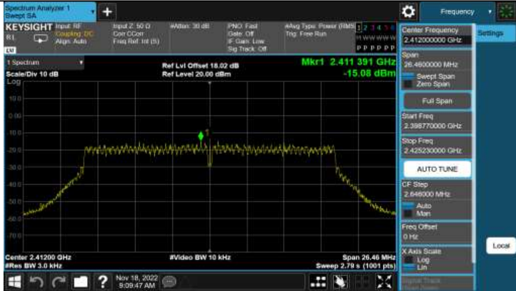
11N20SISO_Ant1_2412
