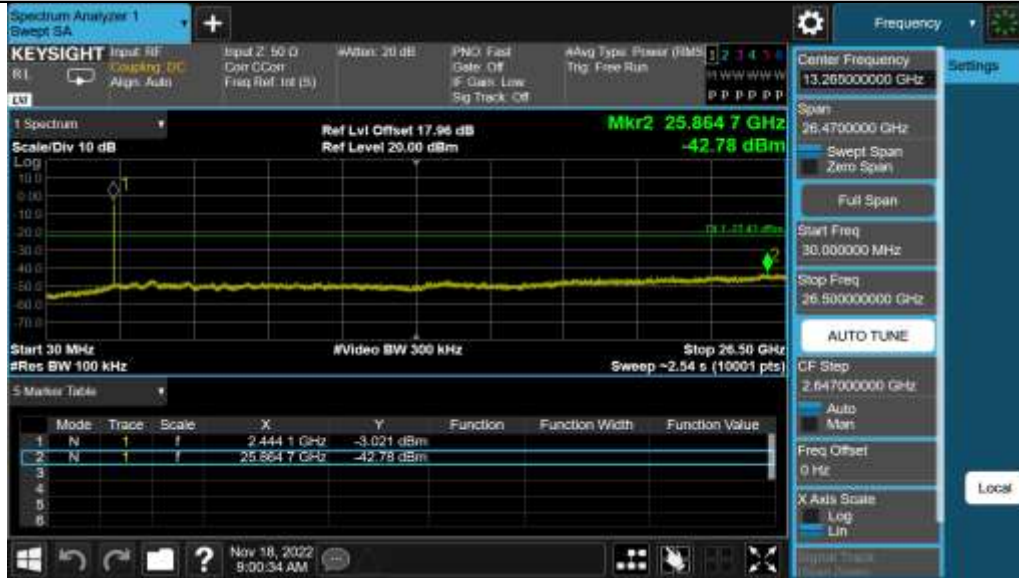
11G_Ant1_2437_30-26500
