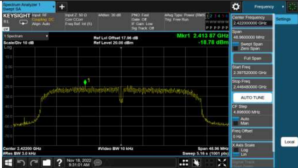
11N40SISO_Ant1_2422
