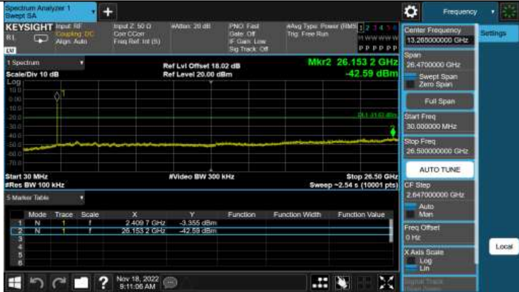
11N20SISO_Ant1_2412_30~26500
