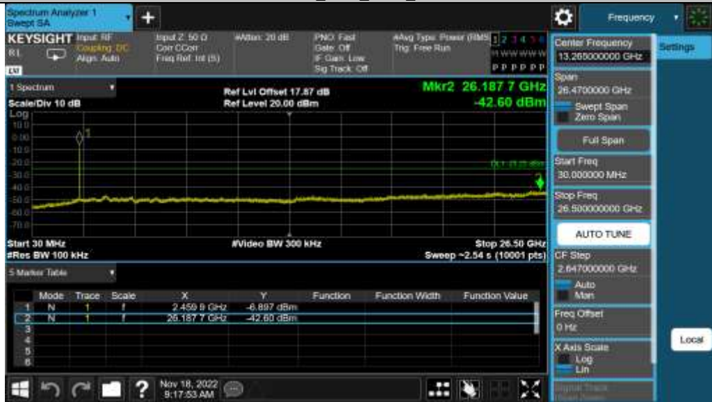
11N20SISO_Ant1_2462_30~26500
