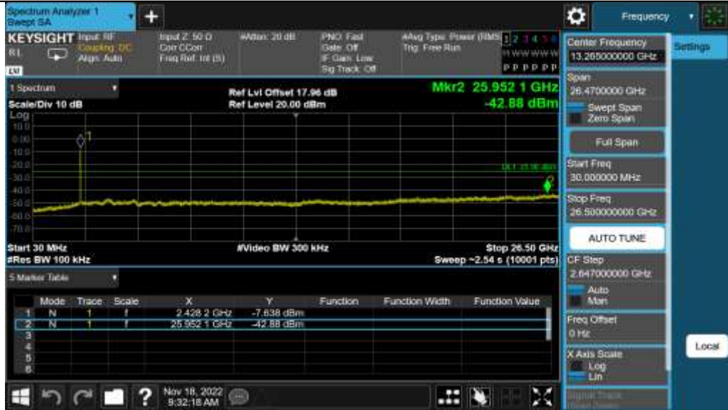
11N40SISO_Ant1_2422_30~26500
