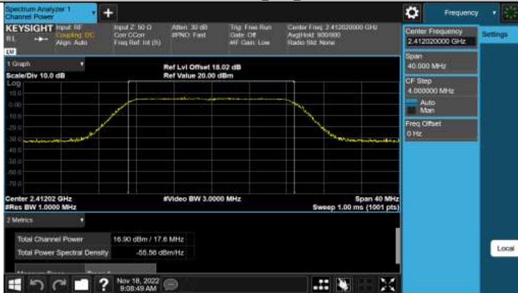
11N20SISO_Ant1_2412
