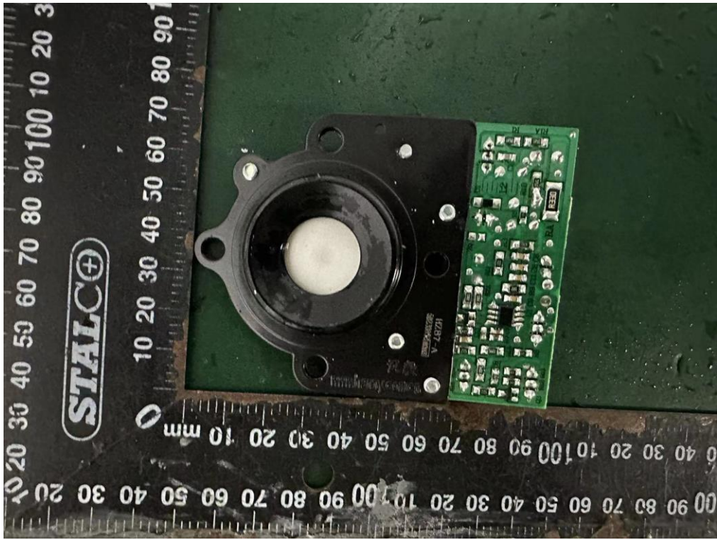
Internal Photos M/N: LUH-M102S-WUS
