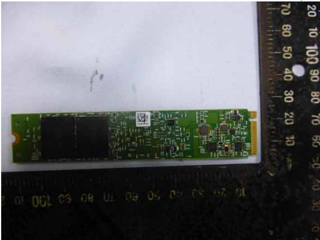
Figure 30 SSD (Solder Side)
