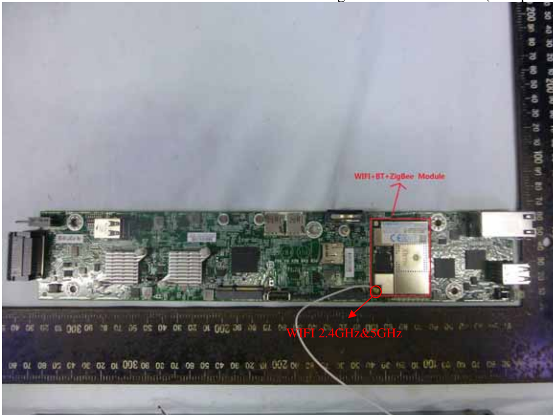
Figure 45 WIFI+BT+ZigBee of PCB Board (Component Side)
