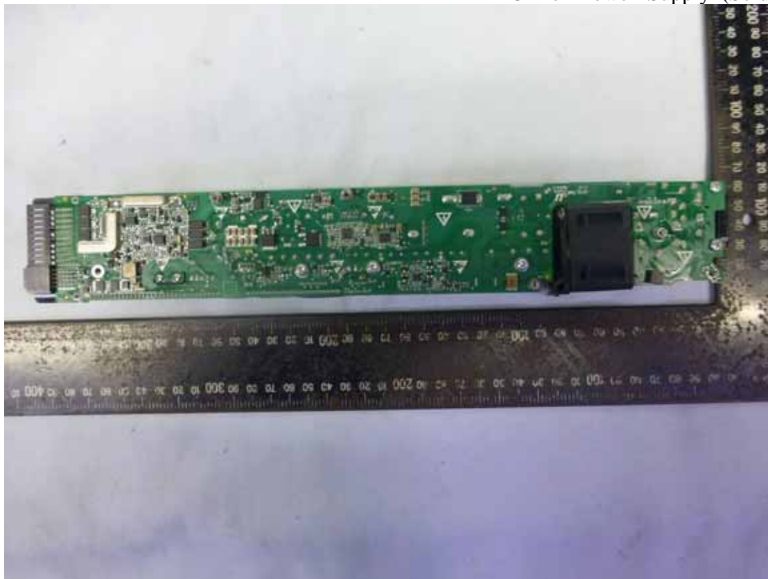
Figure 7 PCB of Power Supply (Solder Side)
