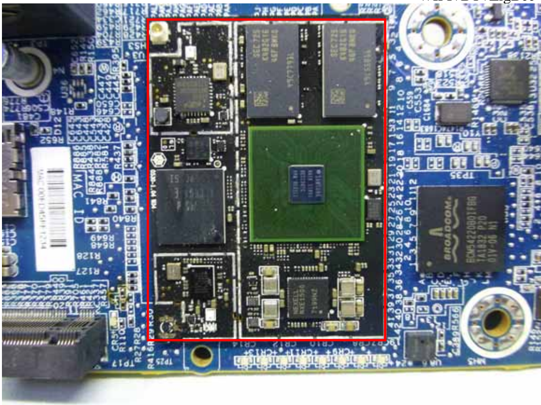
Figure 50 WIFI+BT+ZigBee Module
