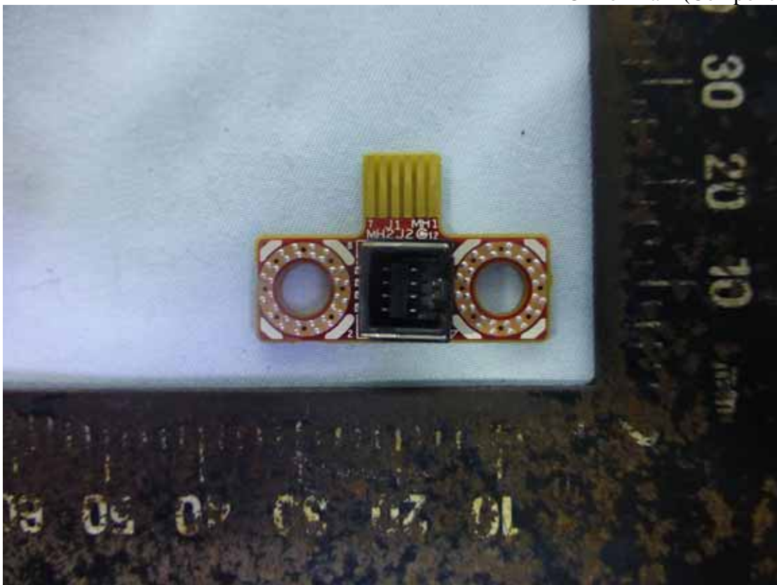
Figure 2 PCB of Fan (Component Side)
