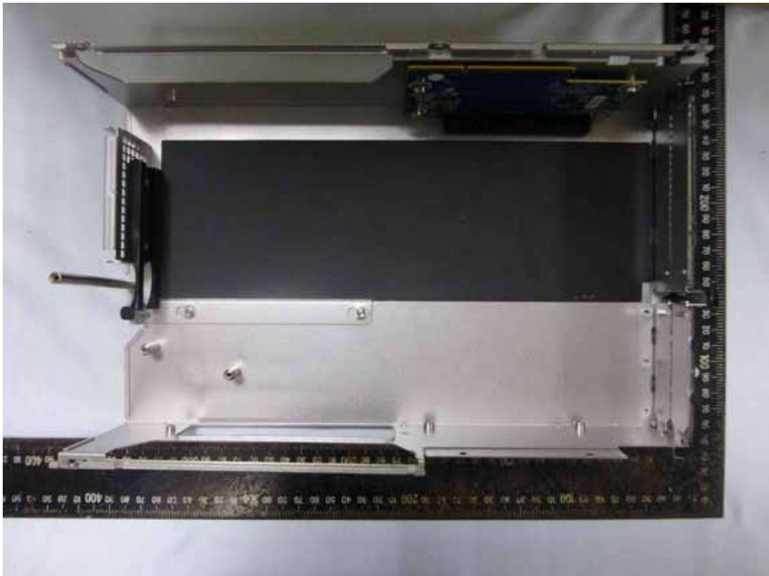
Figure 54 Internal View
