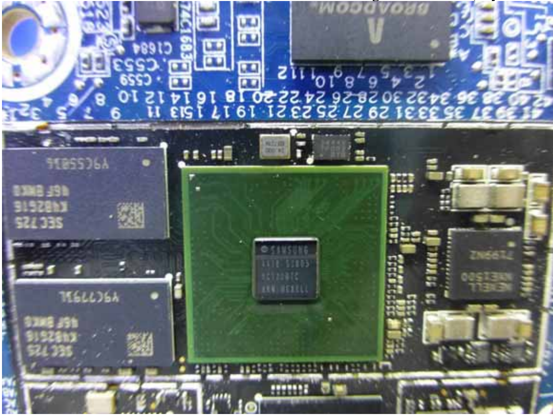
Figure 52 WIFI+BT+ZigBee Module (Crystal Oscillation)
