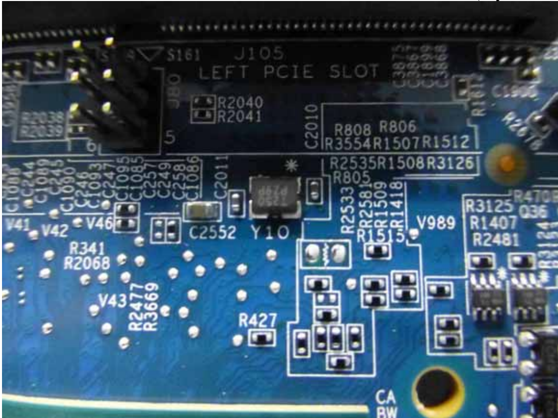
Figure 17 Main Board (Crystal Oscillation)
