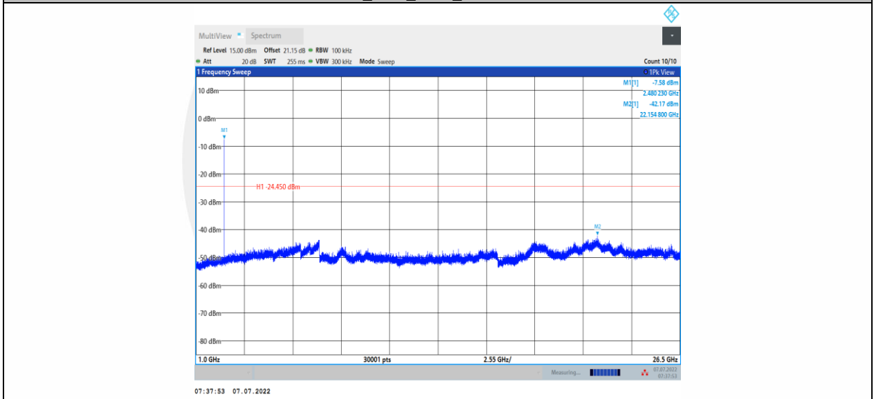
3DH5_Ant1_2480_1000~26500
