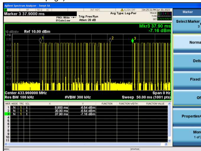
(Transmit cycle 29.00ms)
