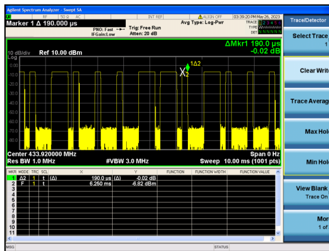
(Time per burst: 0.19ms*16pcs)
