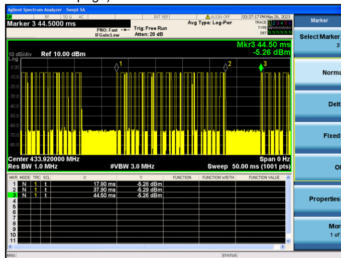
(Transmit cycle 26.70ms)
