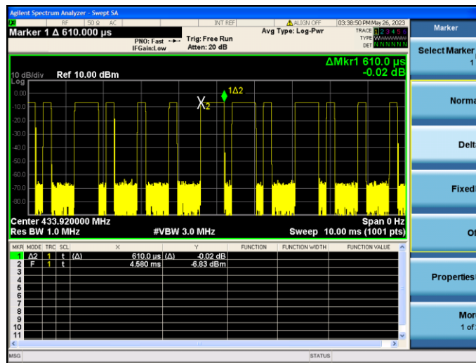
(Time per burst: 0.61ms*9pcs)
