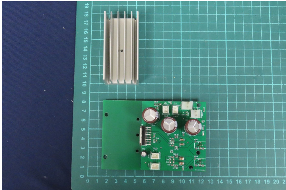
(39) EUT Photo
