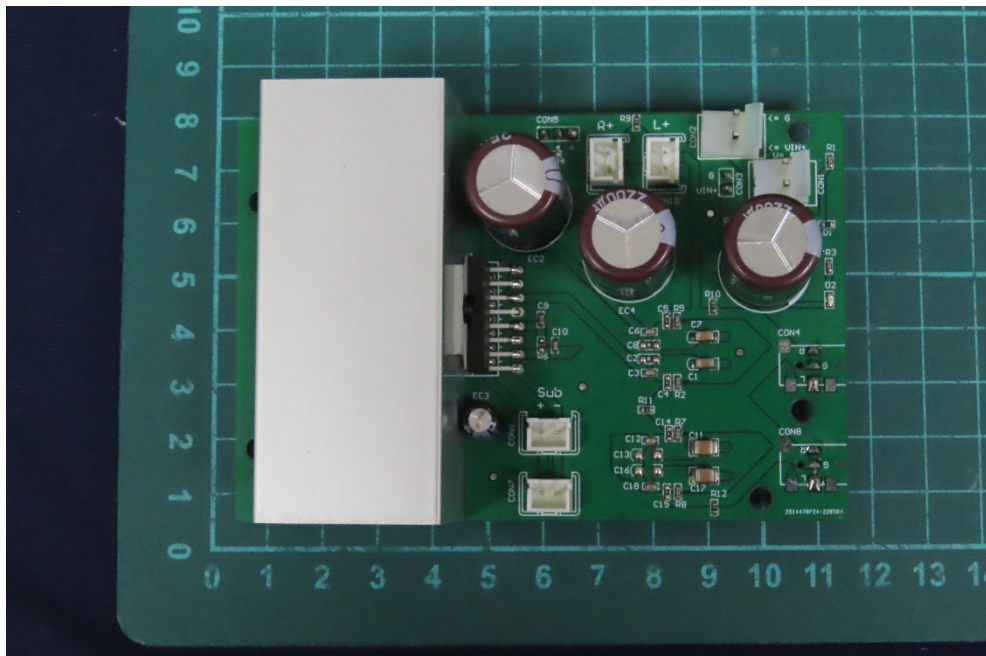
(38) EUT Photo
