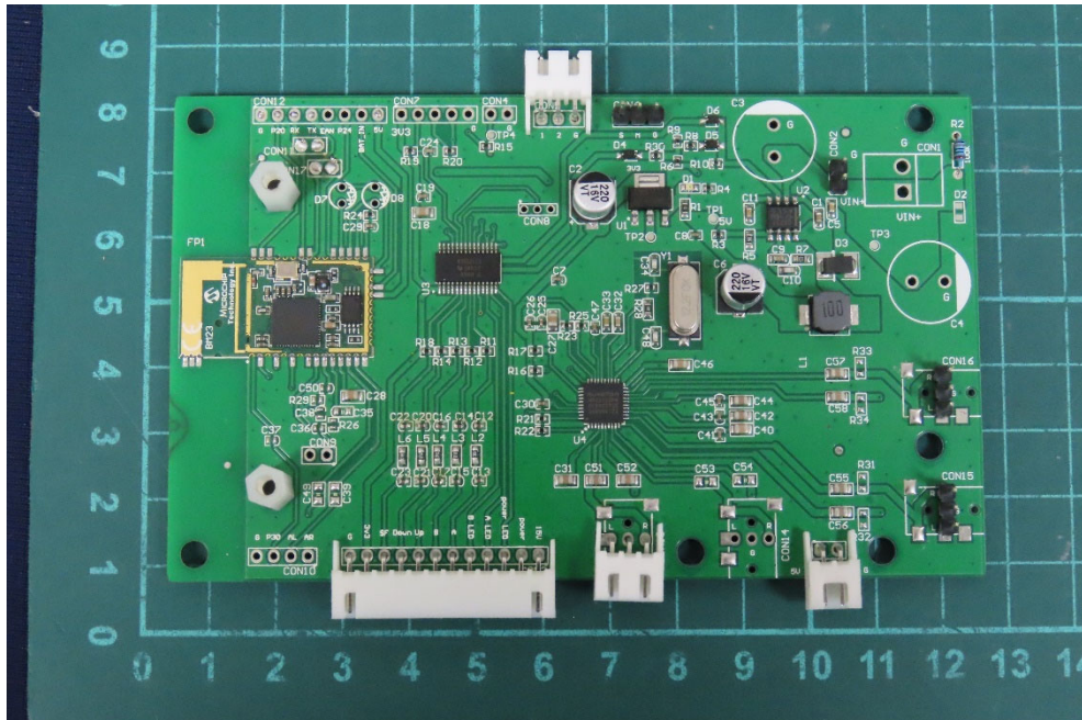
(42) EUT Photo
