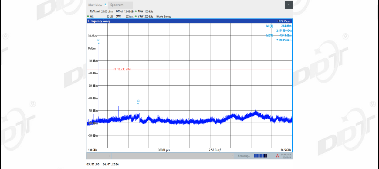
2.4G SRD_Ant1_2476_0~Reference
