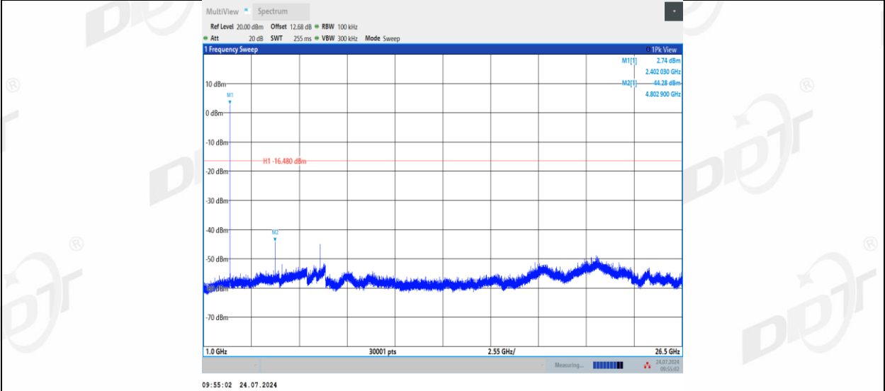
2.4G SRD_Ant1_2444_0~Reference
