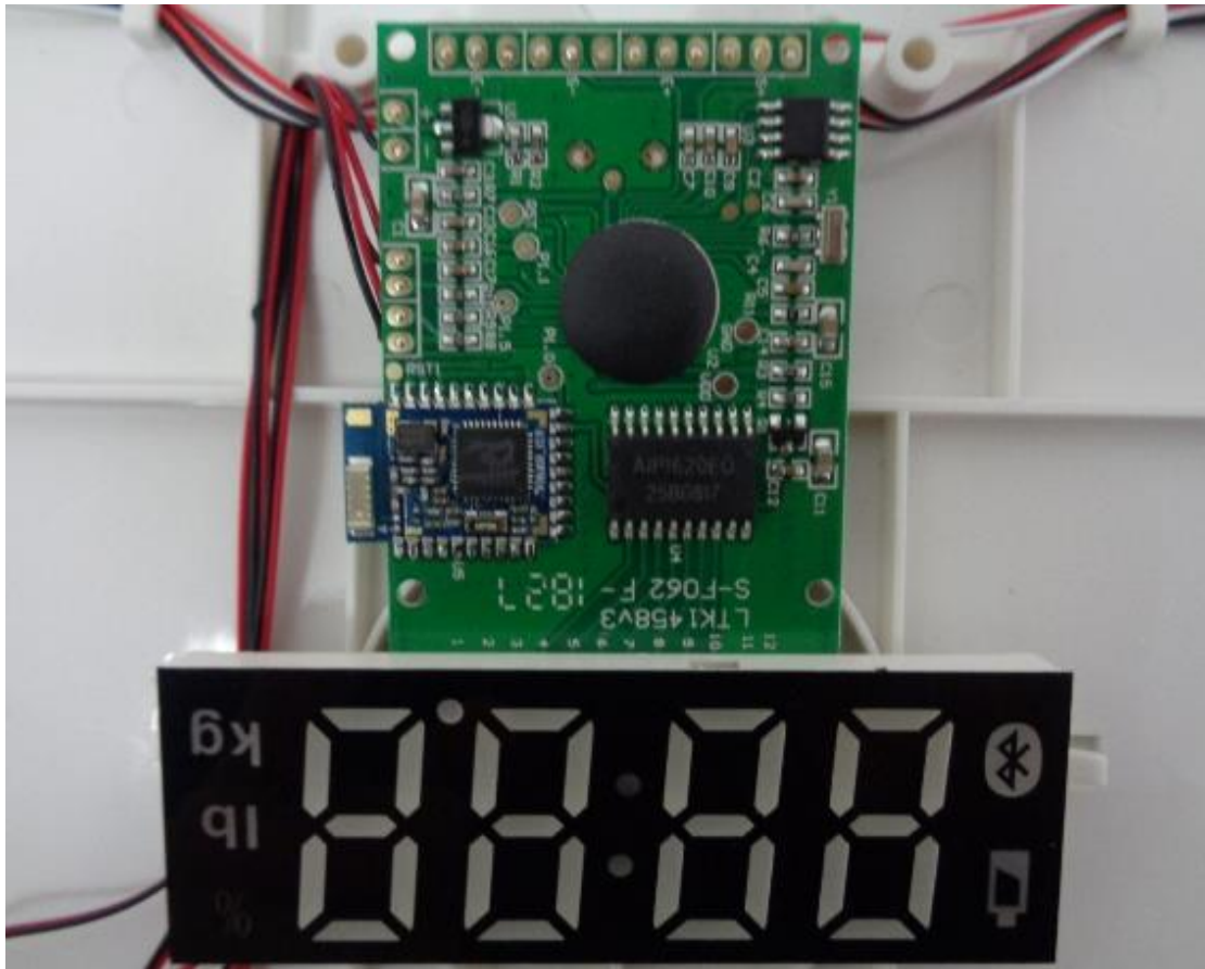
Pic.7: PCB
