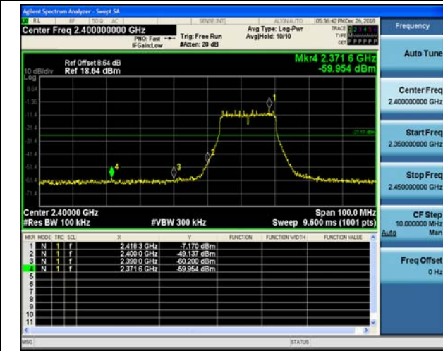
Spurious emission
