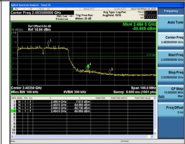
Spurious emission
