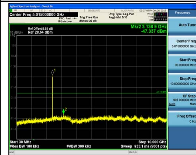
Spurious emission
