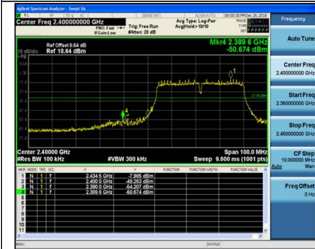
Spurious emission
