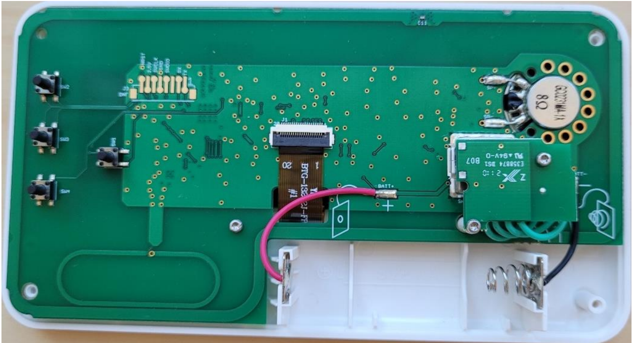
Inside – PCB front view
