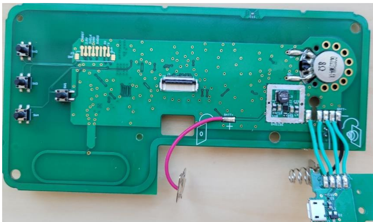
PCB – back view without the shieldbox
