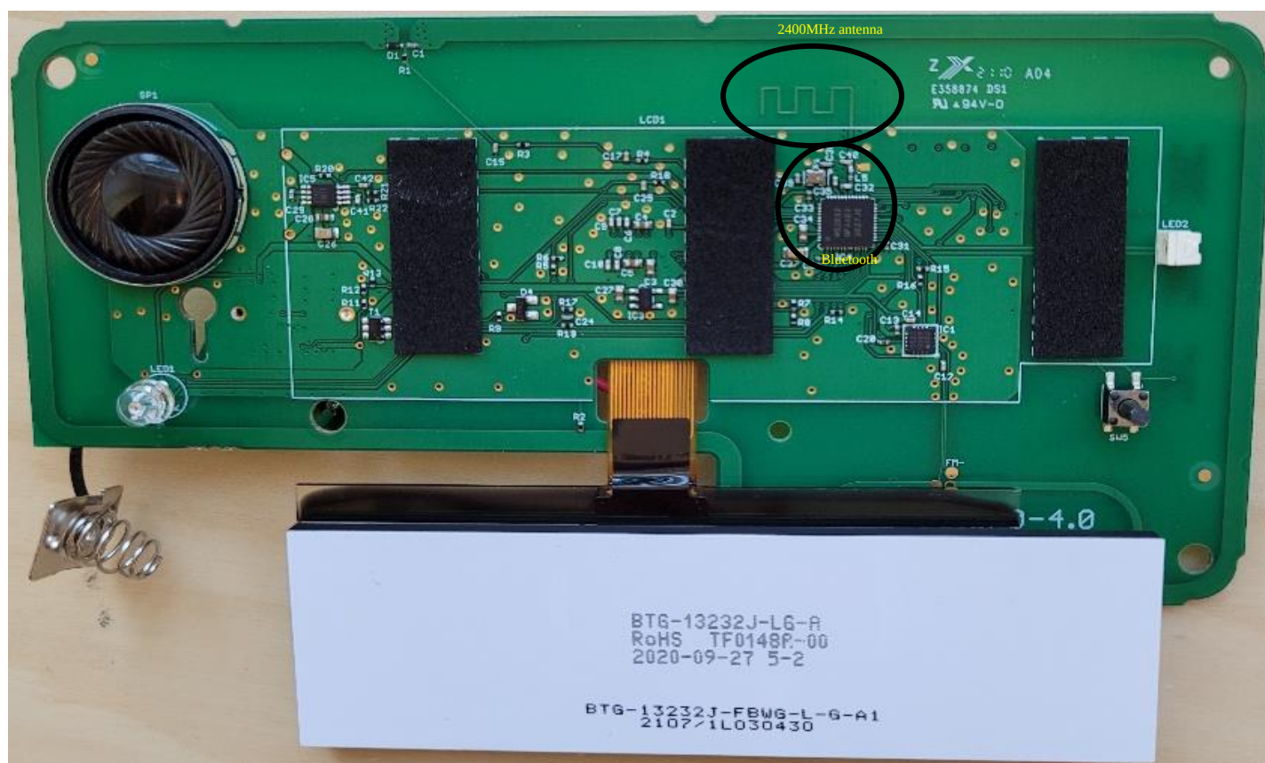
Antenna and BT position
