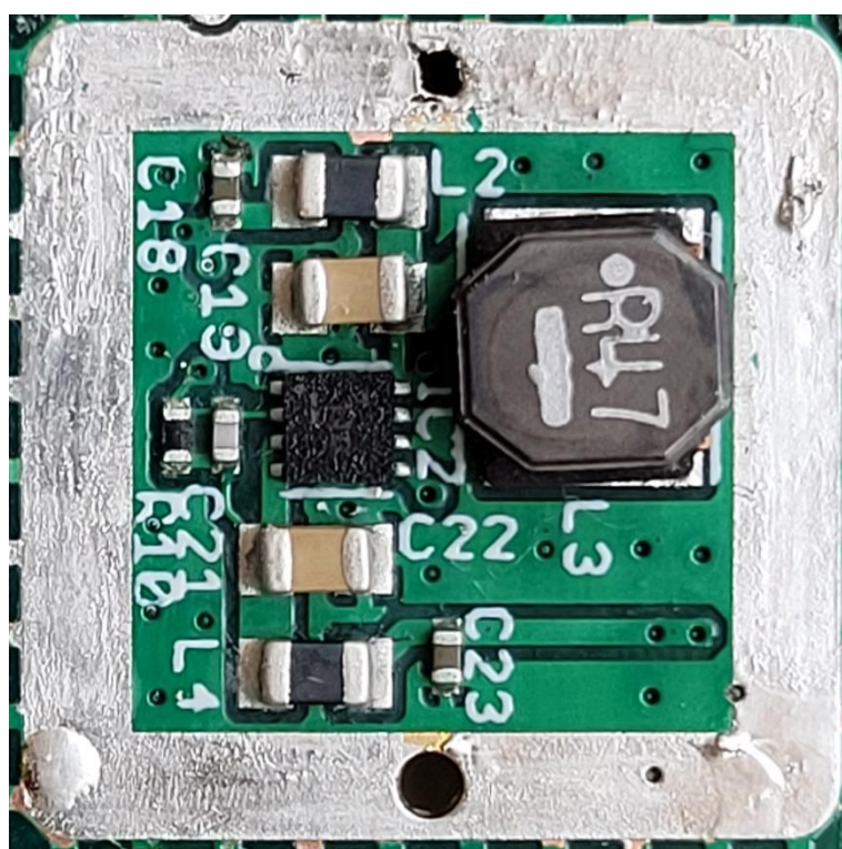
Inside shieldbox
