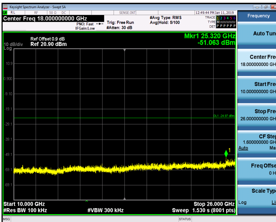
RF Conducted Spurious Emissions_2DH5_2402
