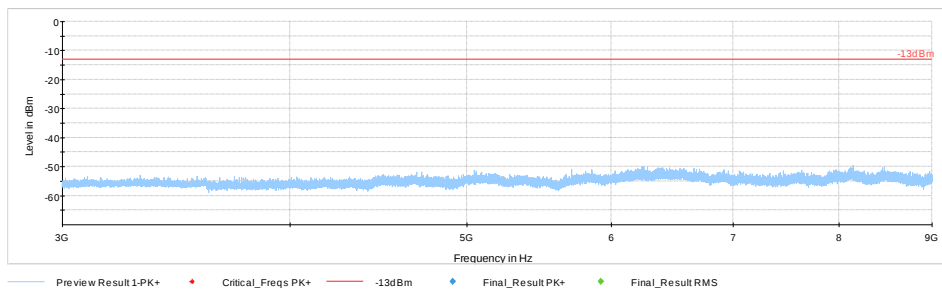
Plot #17 Radiated Emissions: 3-9 GHz
