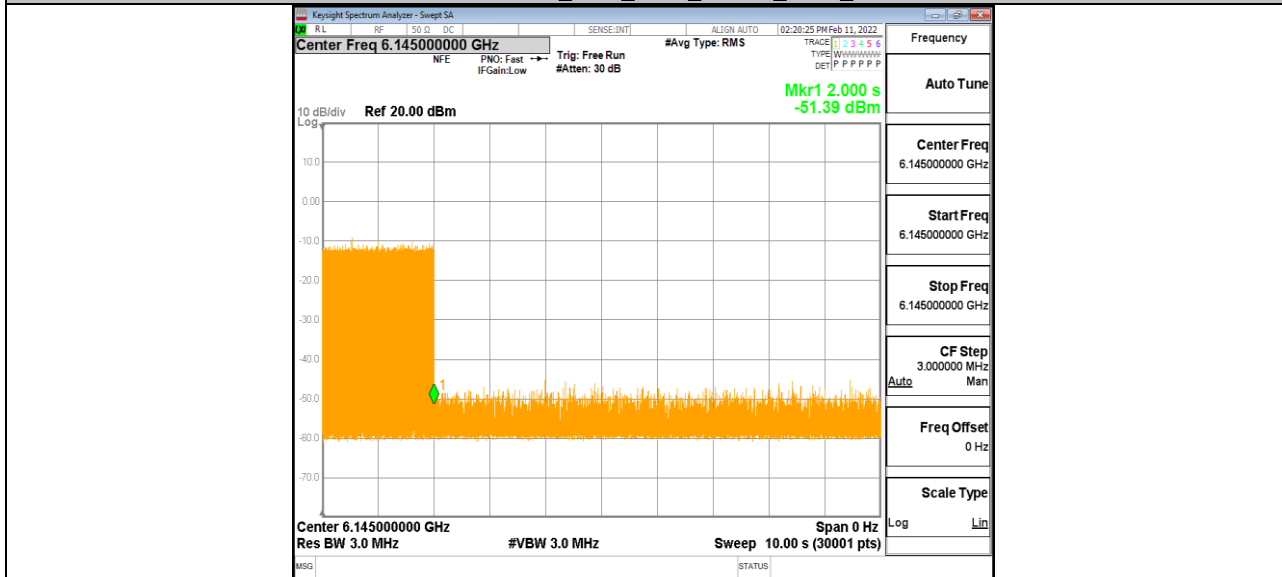
11AX80MIMO_Ant1_6145_Low_6180_1
