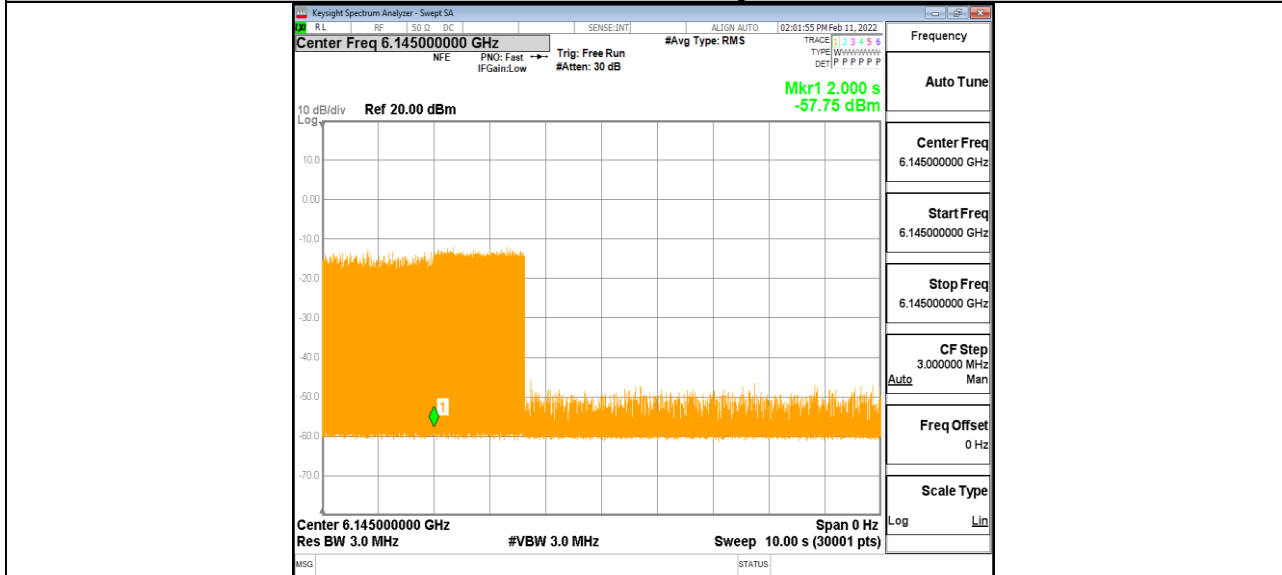
11AX80MIMO_Ant1_6145_Center_6145_1
