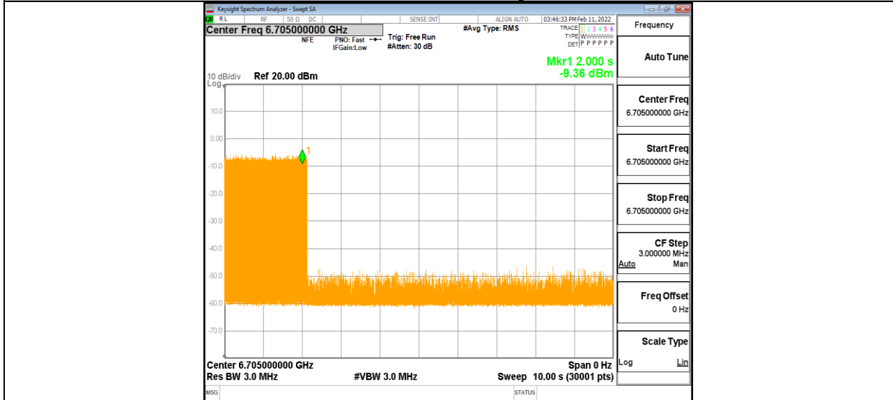
11AX80MIMO_Ant1_6705_High_6670_5
