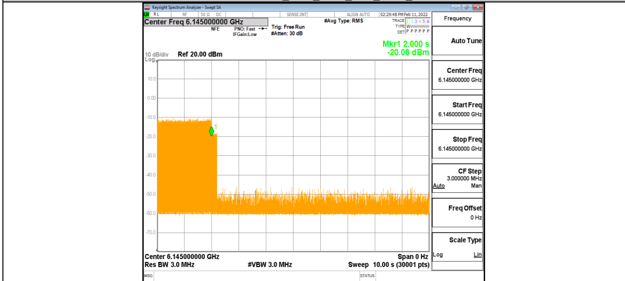
11AX80MIMO Ant1_6145_Low_6180_9
