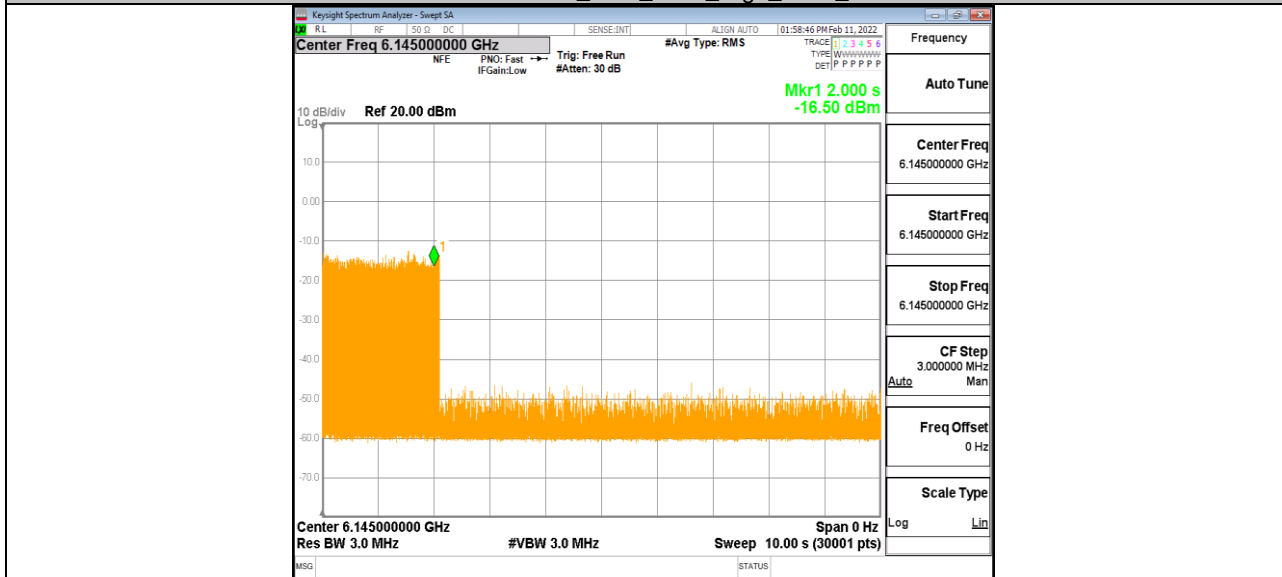
11AX80MIMO_Ant1_6145_High_6110_7
