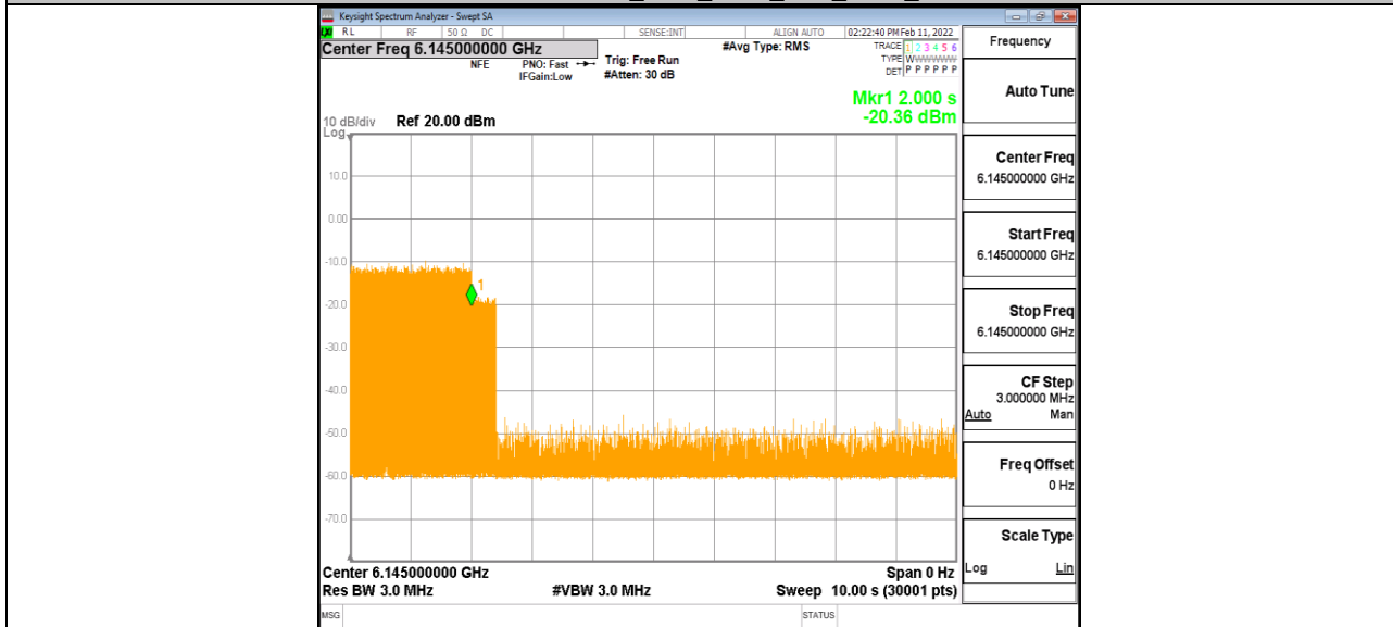
11AX80MIMO_Ant1_6145_Low_6180_3
