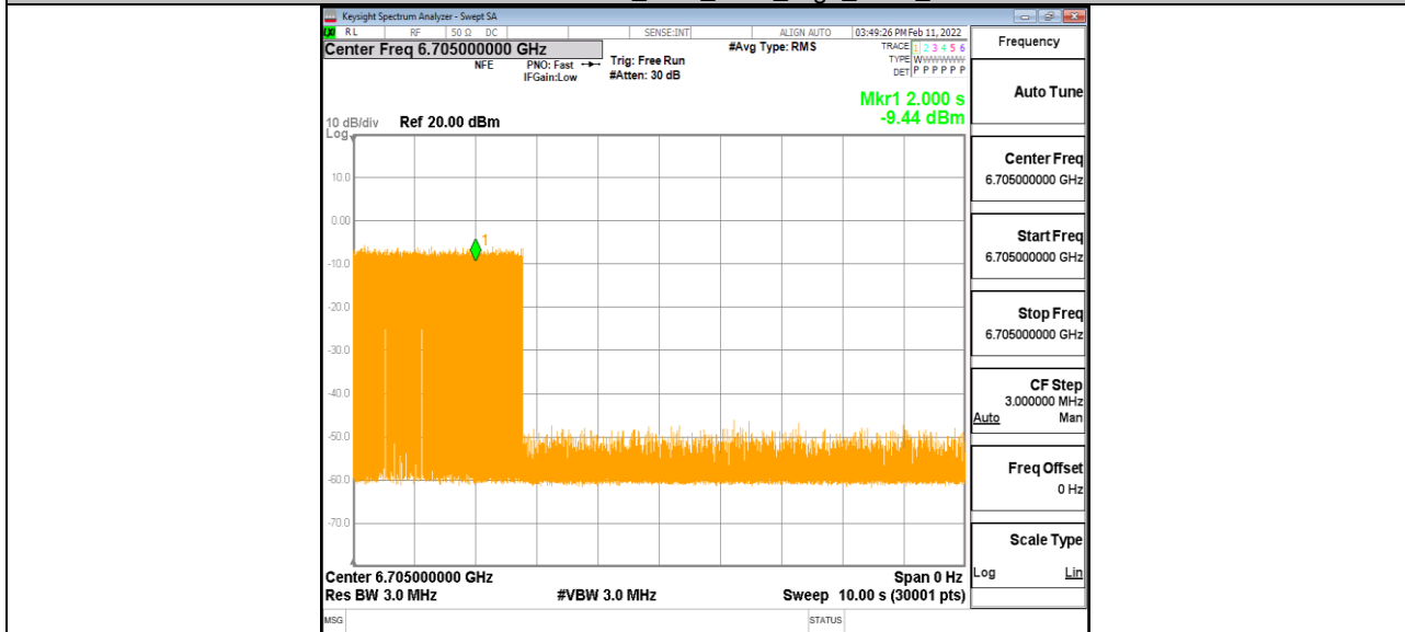
11AX80MIMO_Ant1_6705_High_6670_9
