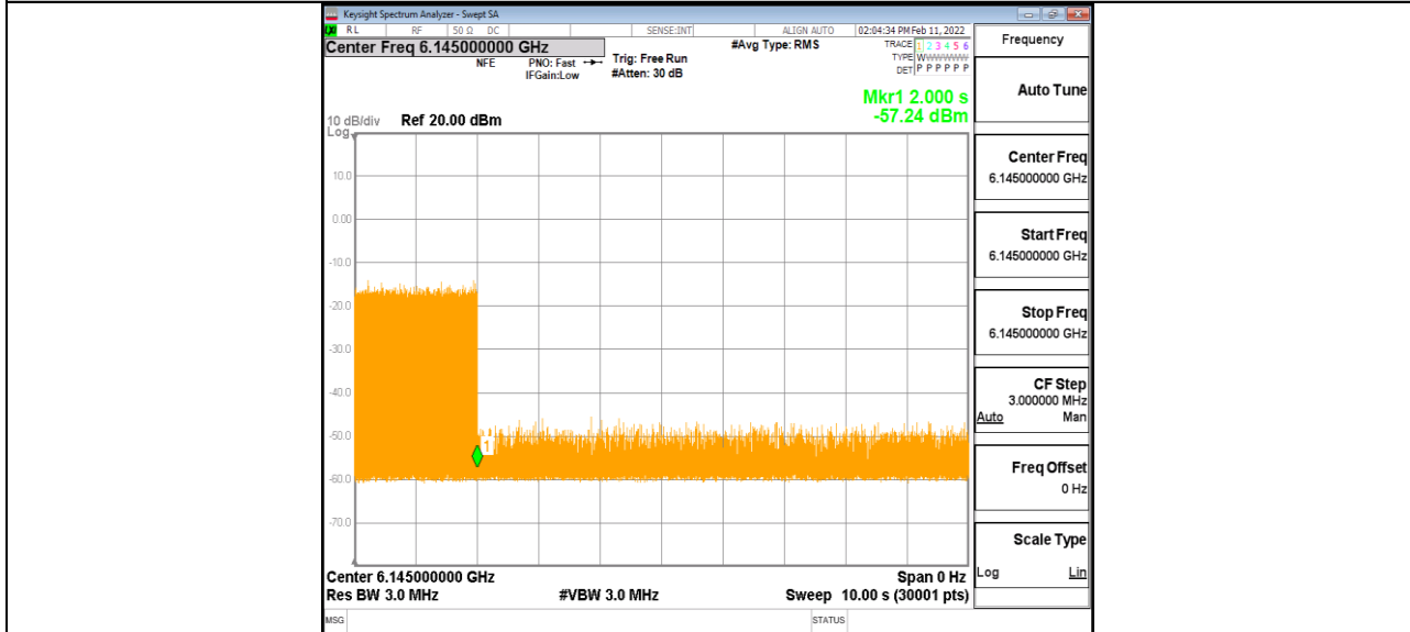
11AX80MIMO_Ant1_6145_Center_6145_3
