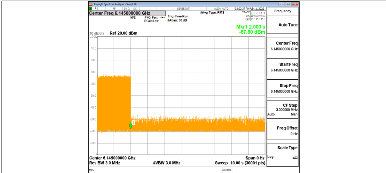
11AX80MIMO_Ant1_6145_Center_6145_2
