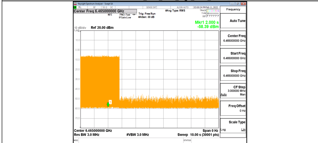
11AX80MIMO_Ant1_6465_High_6430_7
