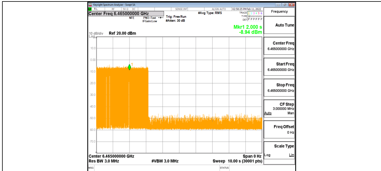
11AX80MIMO_Ant1_6465_High_6430_4
