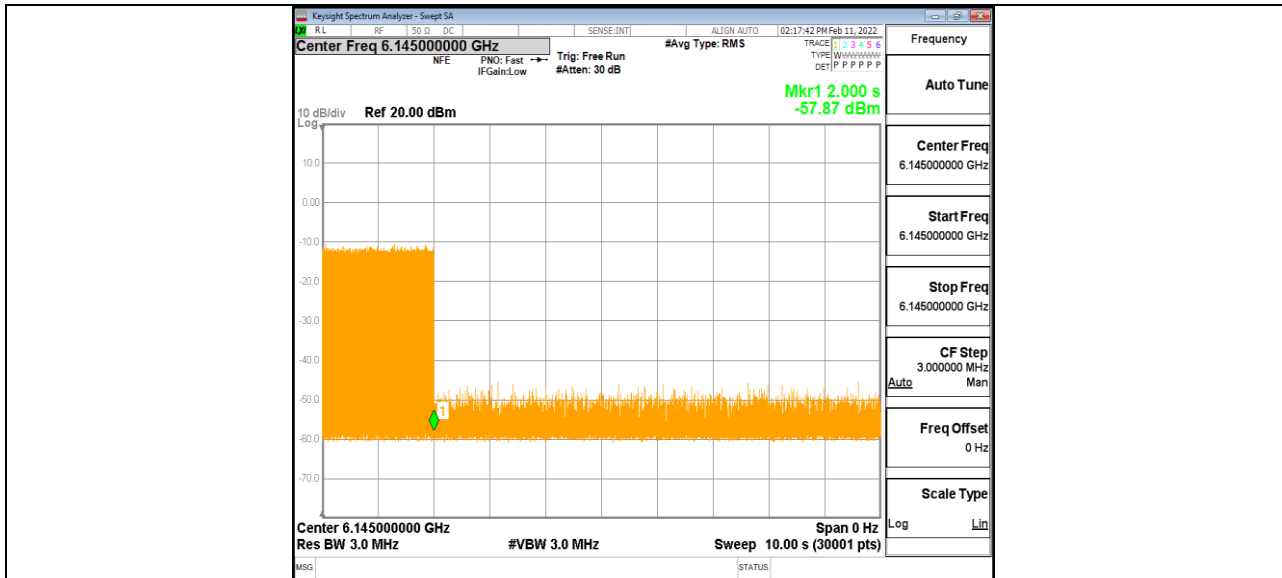
11AX80MIMO_Ant1_6145_Center_6145_6
