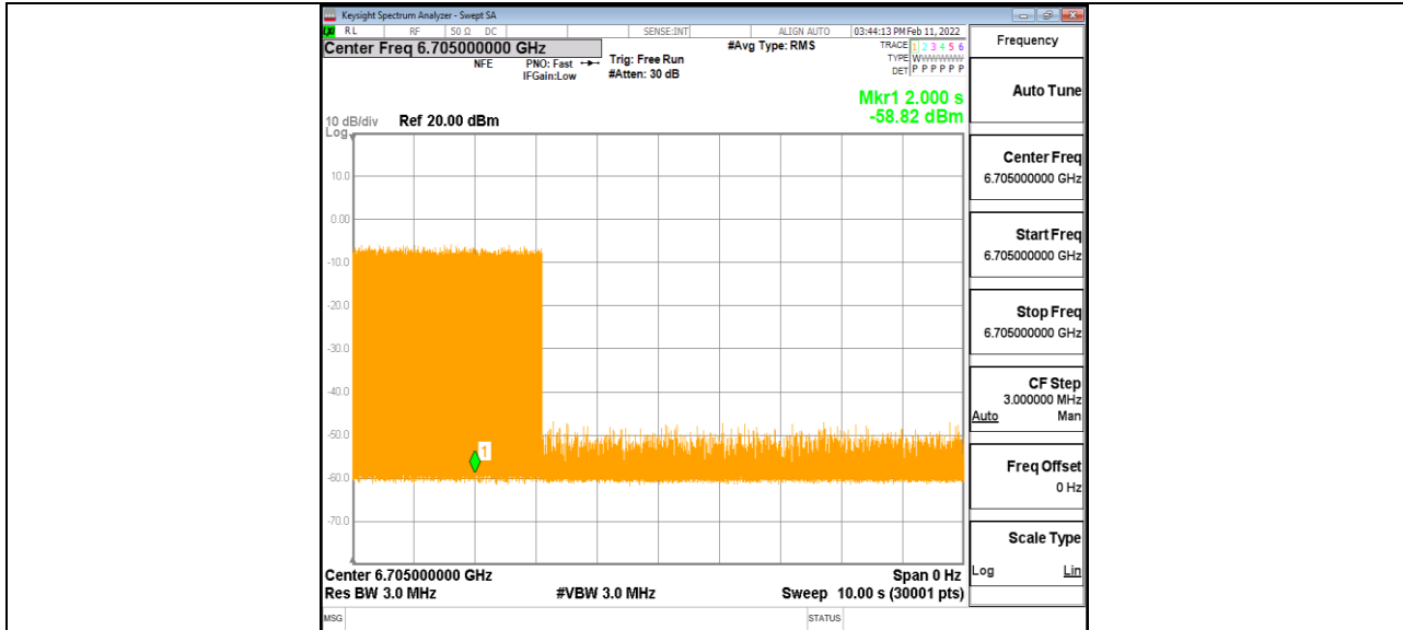
11AX80MIMO_Ant1_6705_High_6670_2
