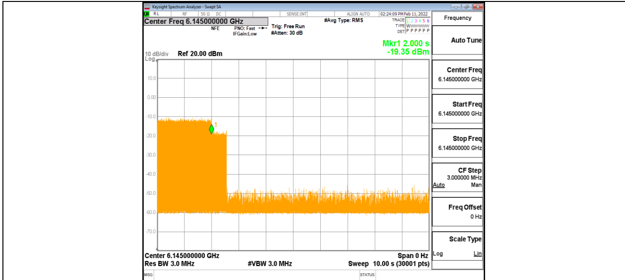
11AX80MIMO_Ant1_6145_Low_6180_4
