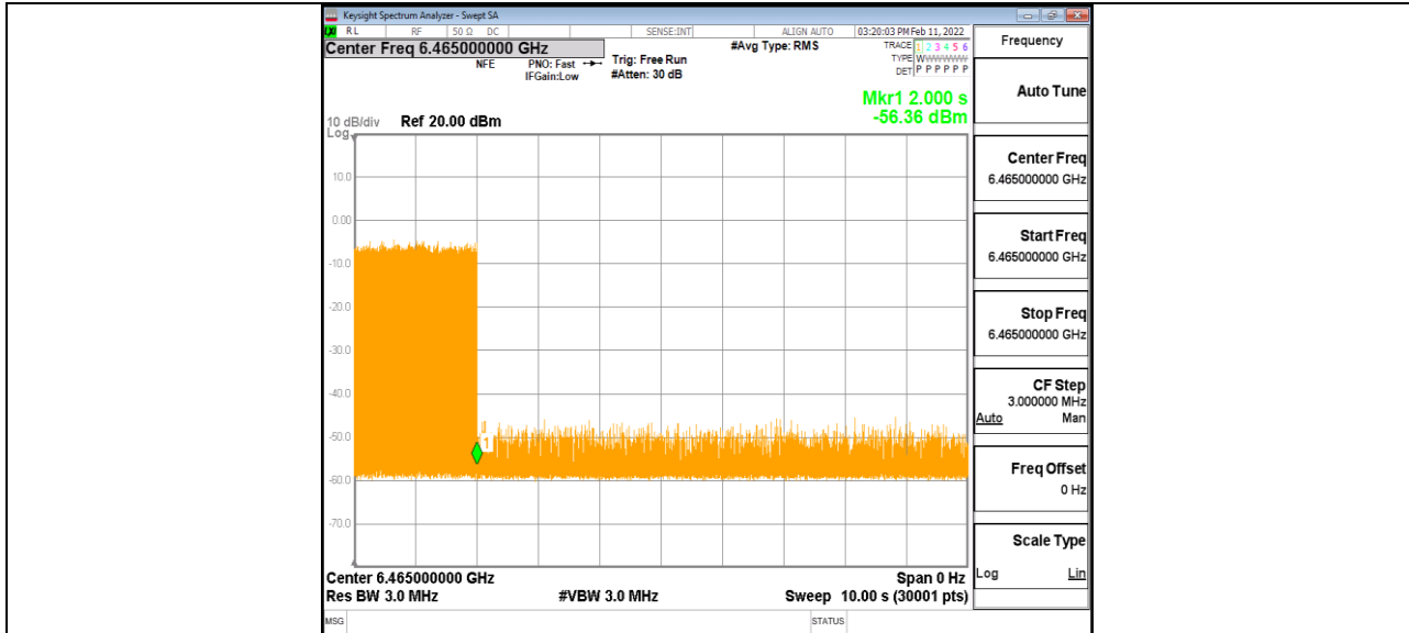
11AX80MIMO Ant1_6465_Low_6500_2
