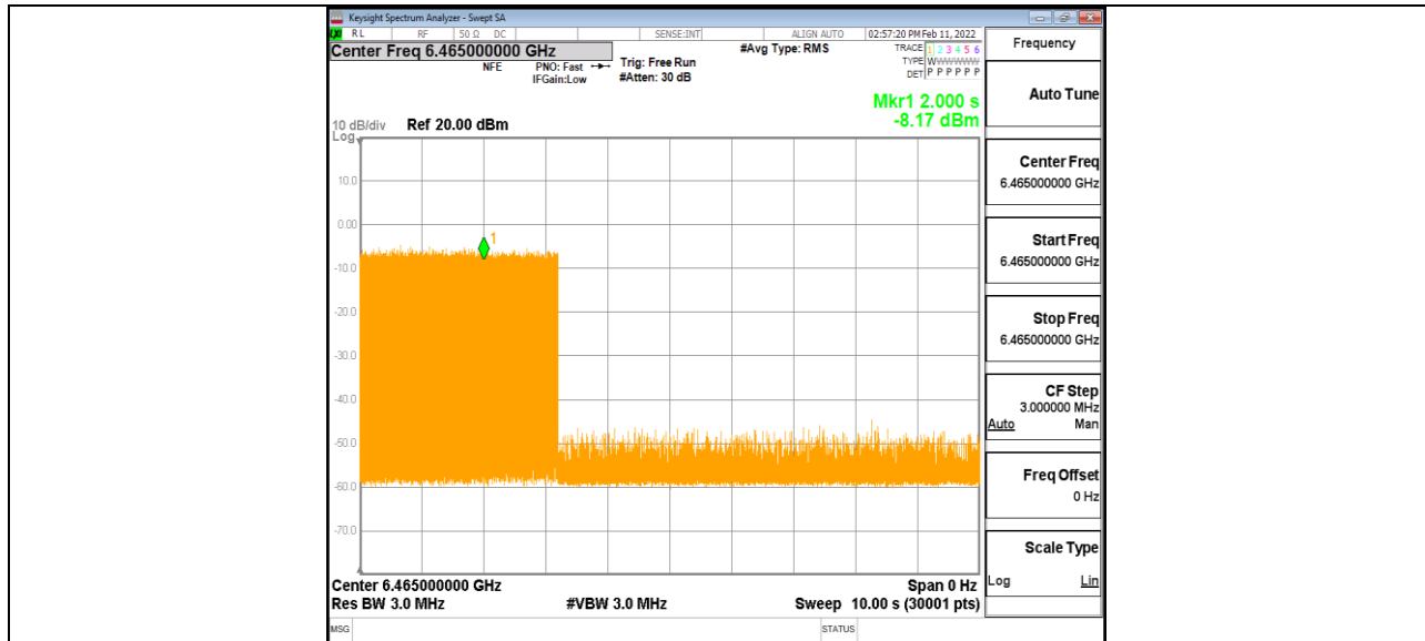
11AX80MIMO_Ant1_6465_High_6430_2
