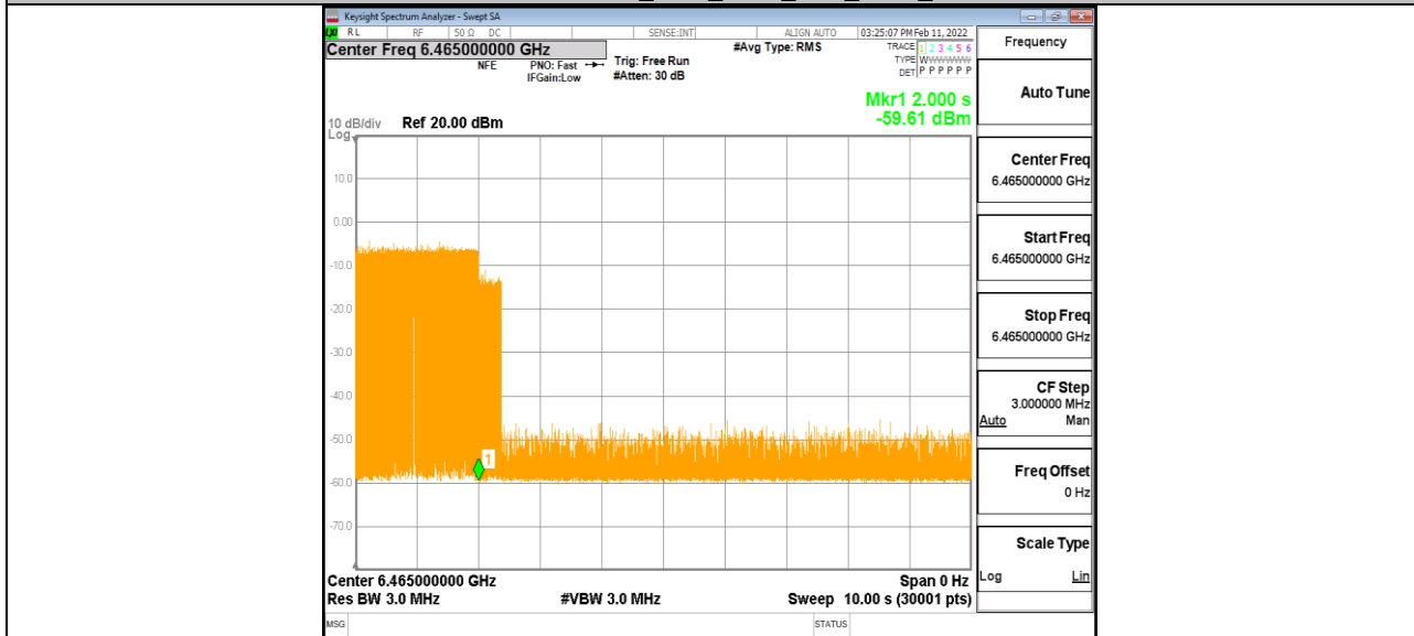
11AX80MIMO Ant1_6465_Low_6500_5
