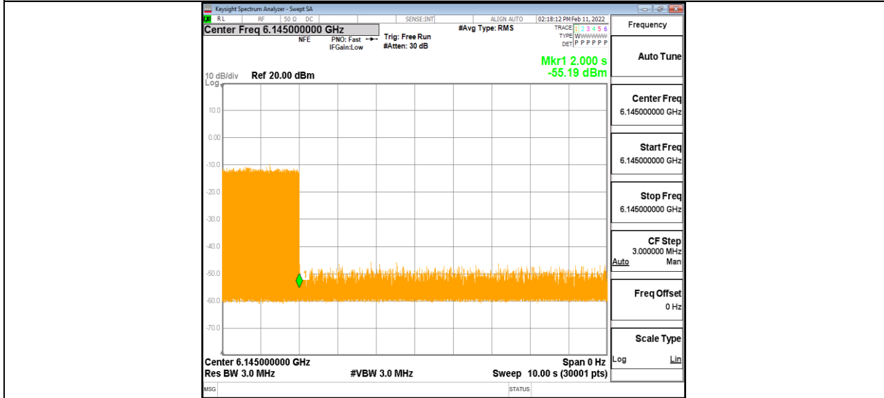
11AX80MIMO_Ant1_6145_Center_6145_7
