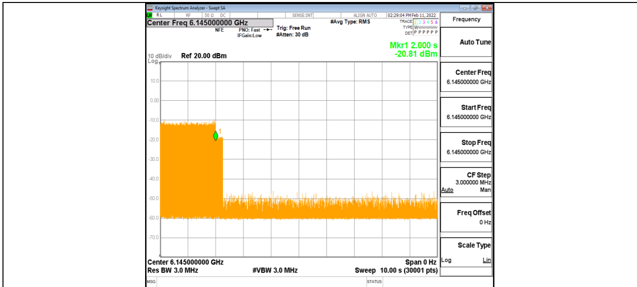
11AX80MIMO Ant1_6145_Low_6180_8
