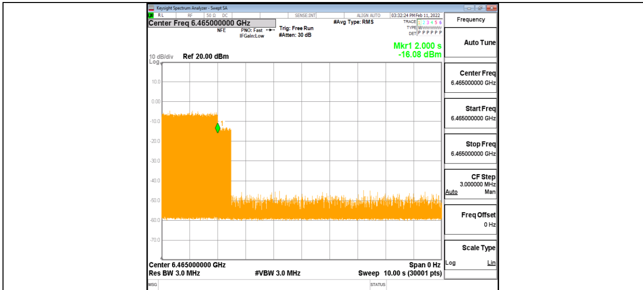
11AX80MIMO_Ant1_6465_Low_6500_10
