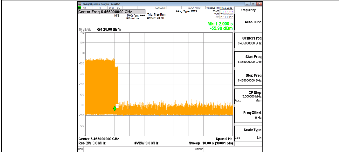
11AX80MIMO_Ant1_6465_Low_6500_7
