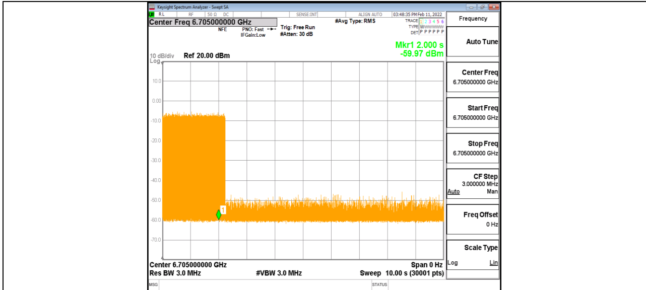
11AX80MIMO_Ant1_6705_High_6670_8
