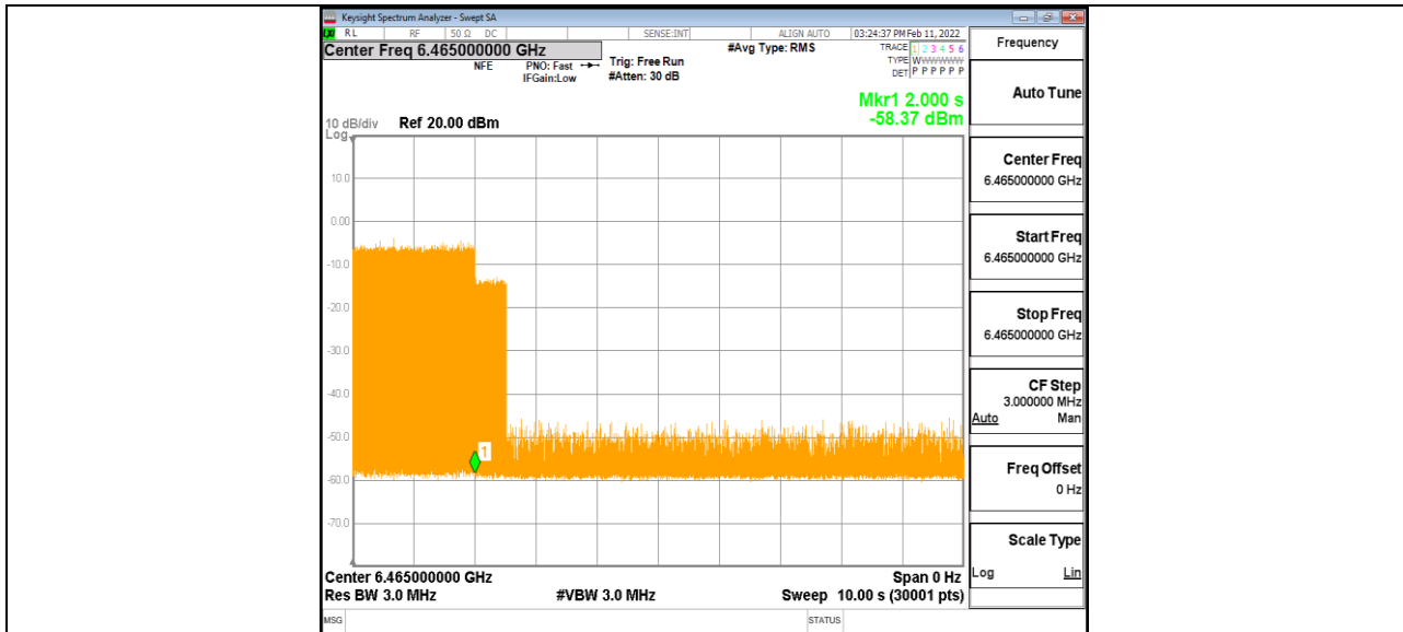
11AX80MIMO Ant1_6465_Low_6500_4
