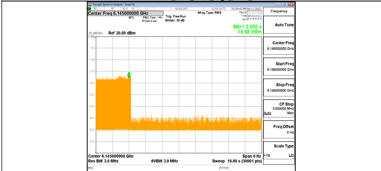
11AX80MIMO_Ant1_6145_High_6110_5
