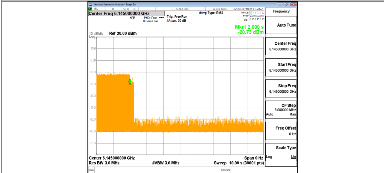
11AX80MIMO Ant1_6145_Low_6180_7
