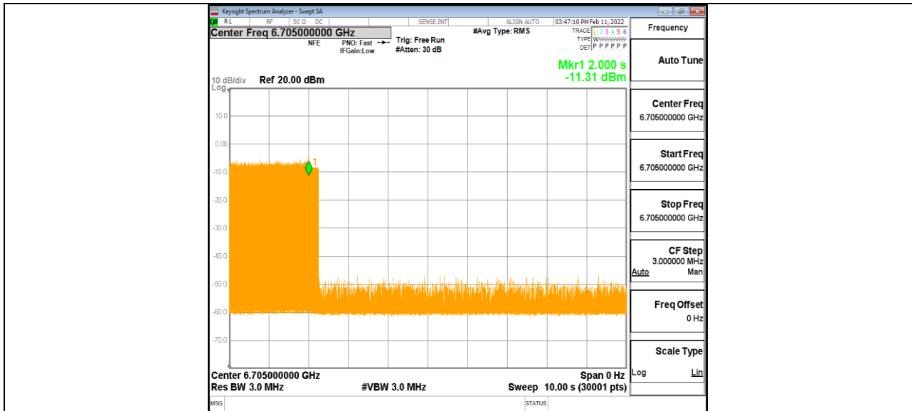
11AX80MIMO_Ant1_6705_High_6670_6
