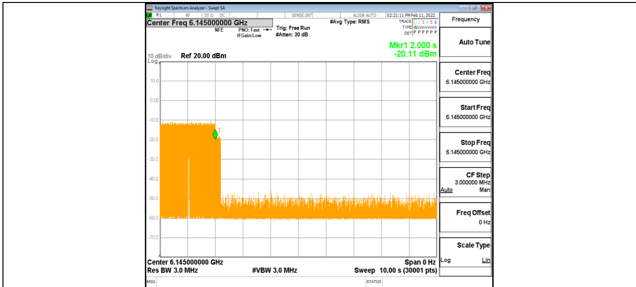
11AX80MIMO_Ant1_6145_Low_6180_2
