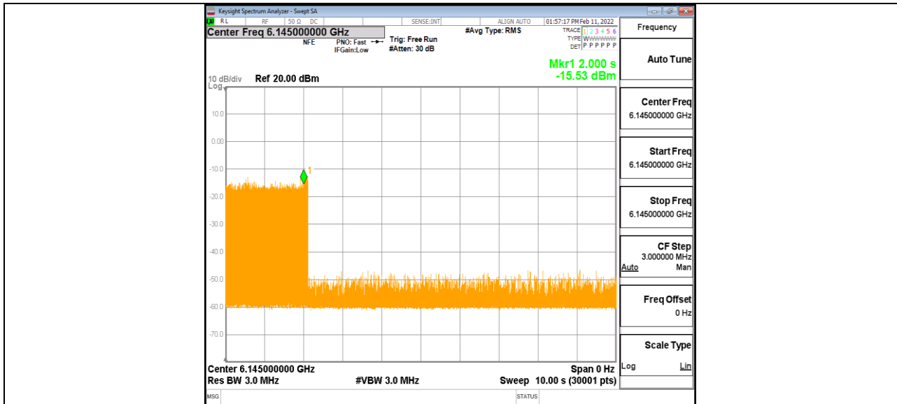
11AX80MIMO_Ant1_6145_High_6110_6
