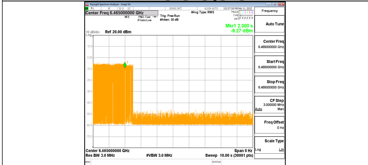
11AX80MIMO_Ant1_6465_High_6430_3
