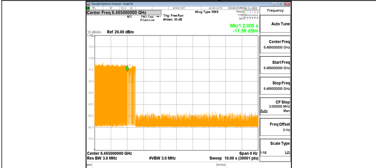
11AX80MIMO_Ant1_6465_High_6430_9
