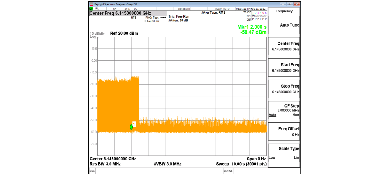
11AX80MIMO_Ant1_6145_High_6110_10
