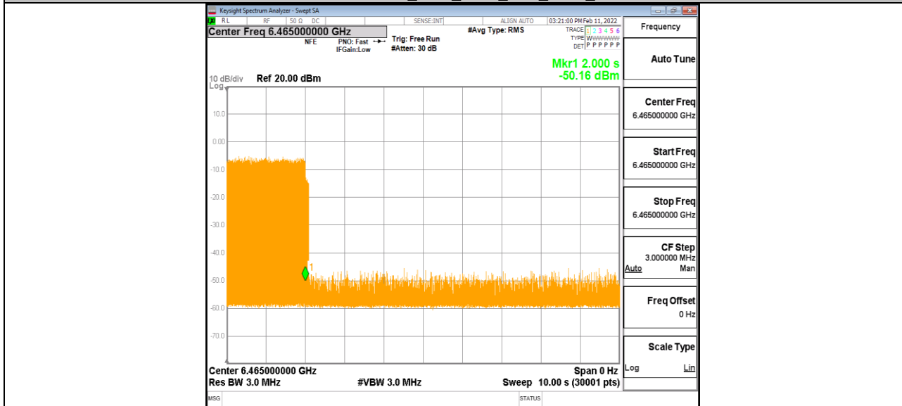
11AX80MIMO Ant1_6465_Low_6500_3
