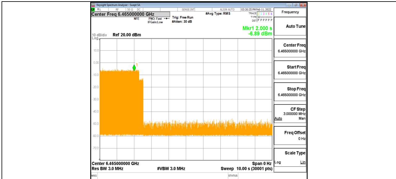
11AX80MIMO Ant1_6465_Low_6500_8
