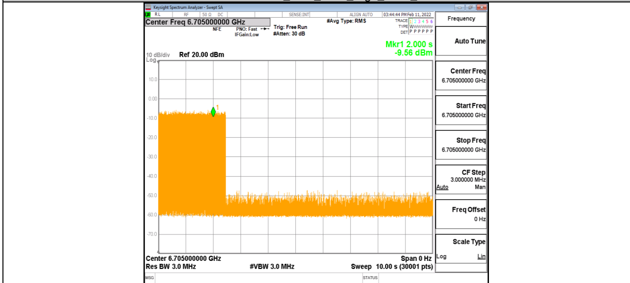
11AX80MIMO_Ant1_6705_High_6670_3
