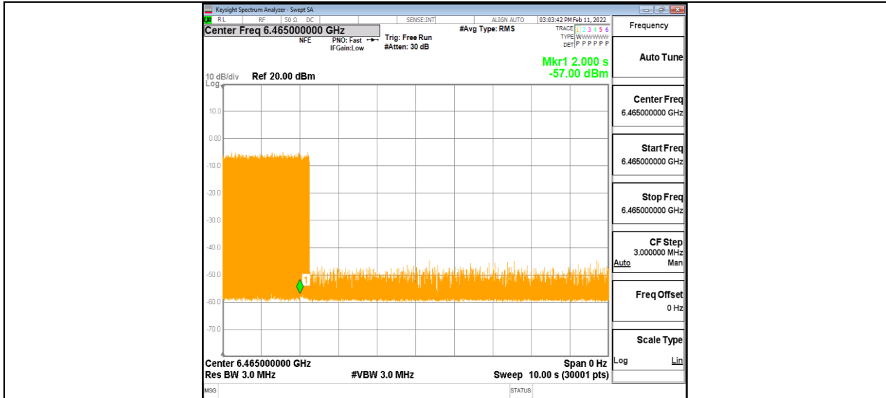
11AX80MIMO_Ant1_6465_High_6430_8
