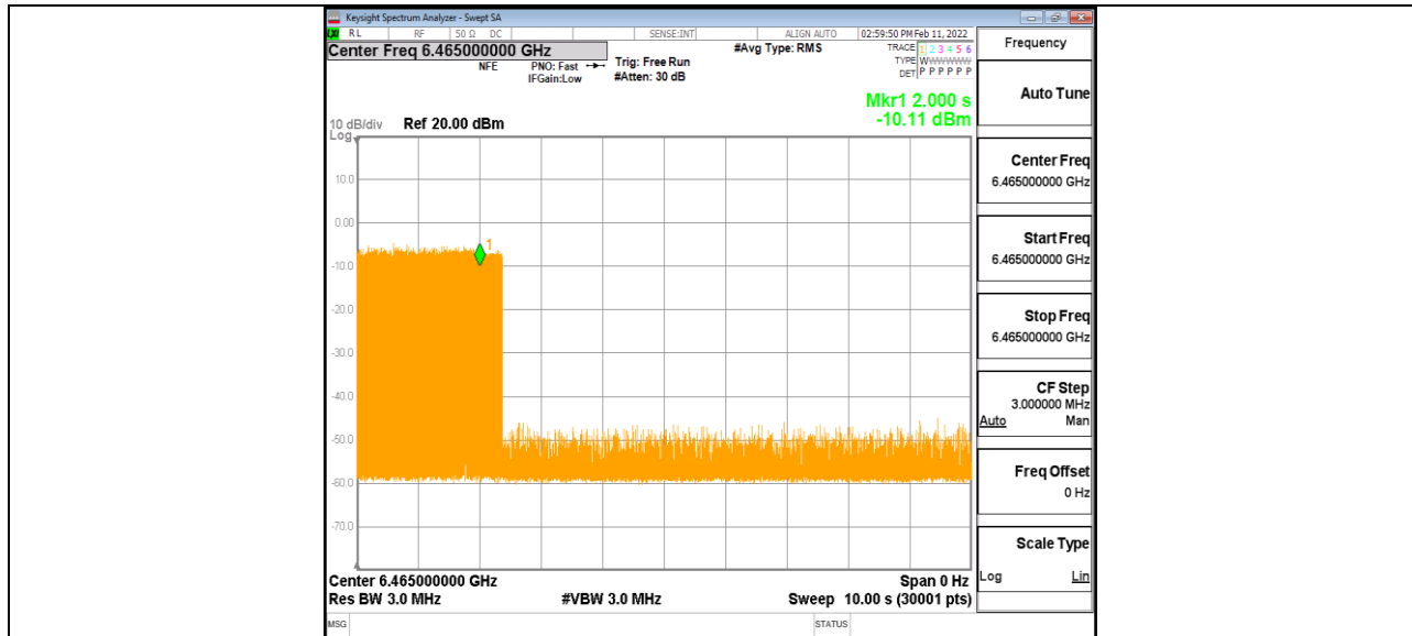
11AX80MIMO_Ant1_6465_High_6430_6
