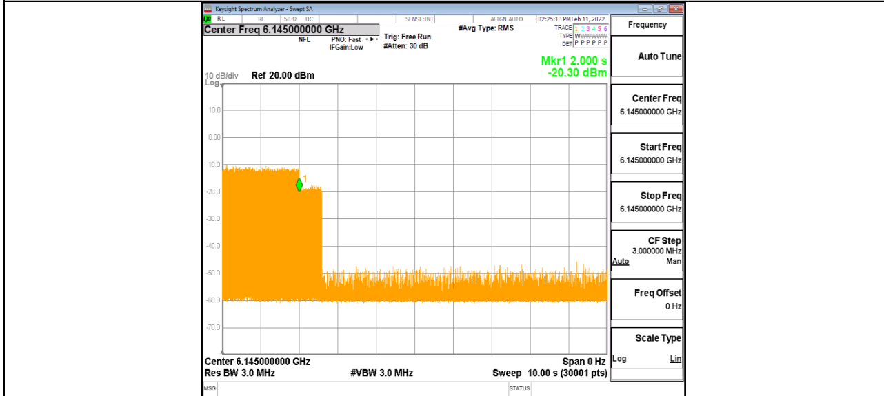
11AX80MIMO_Ant1_6145_Low_6180_5
