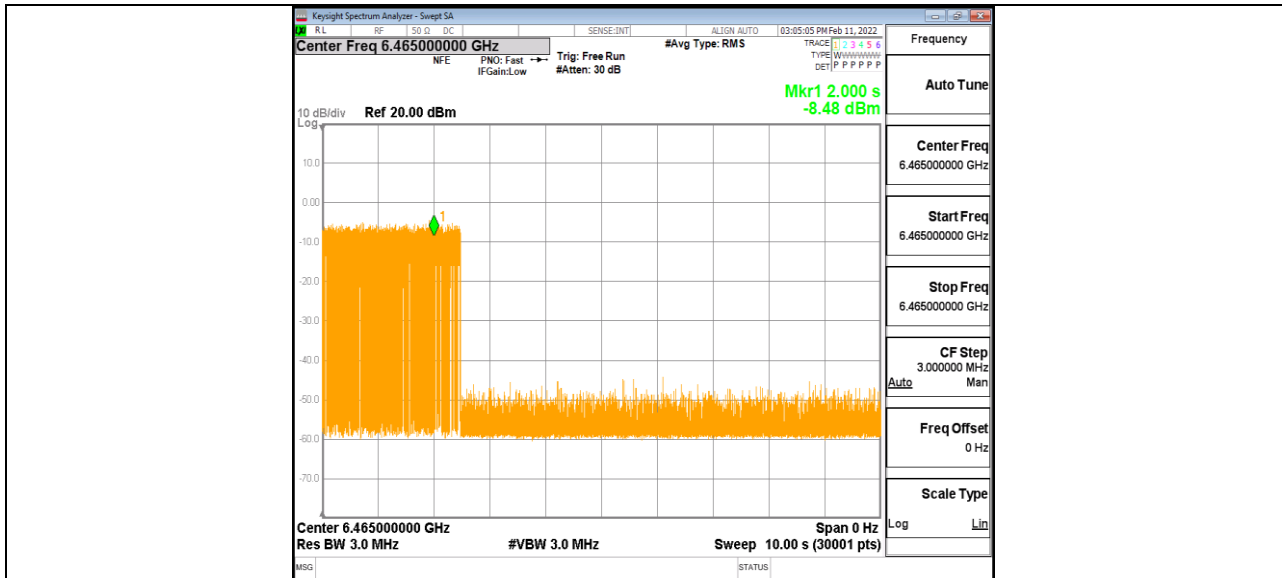
11AX80MIMO_Ant1_6465_High_6430_10
