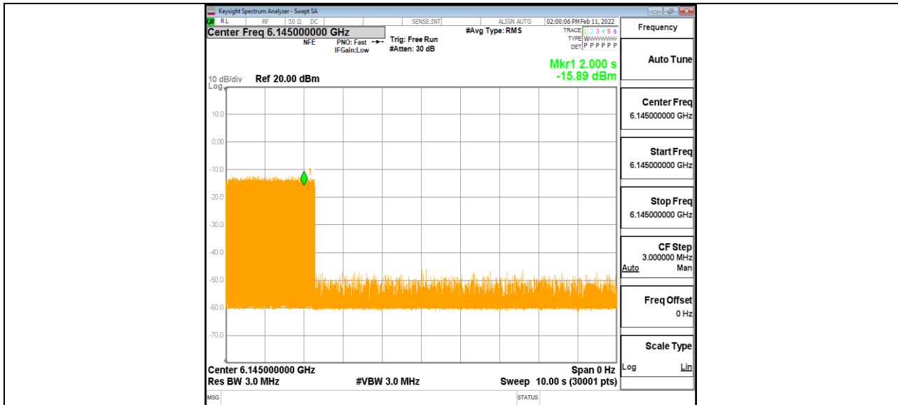
11AX80MIMO_Ant1_6145_High_6110_8
