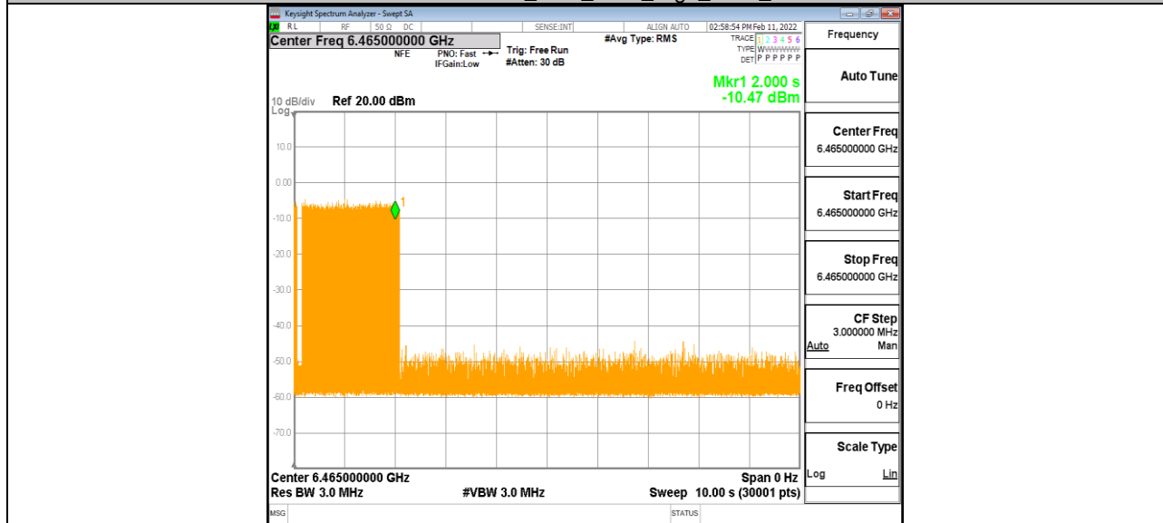
11AX80MIMO_Ant1_6465_High_6430_5
