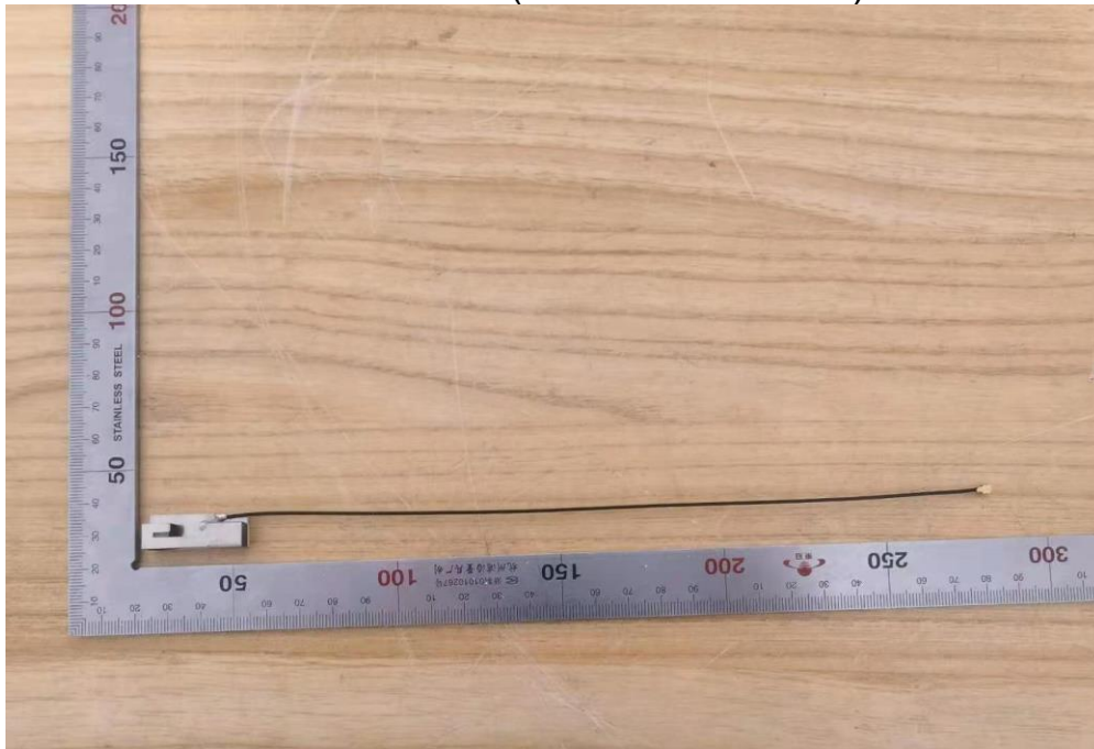
View of EUT-4(BT ANT 2-230mm)
