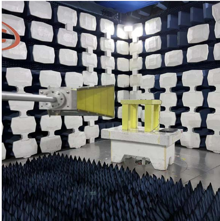
(3) Radiated spurious emission Test Setup(Above 1GHz)
