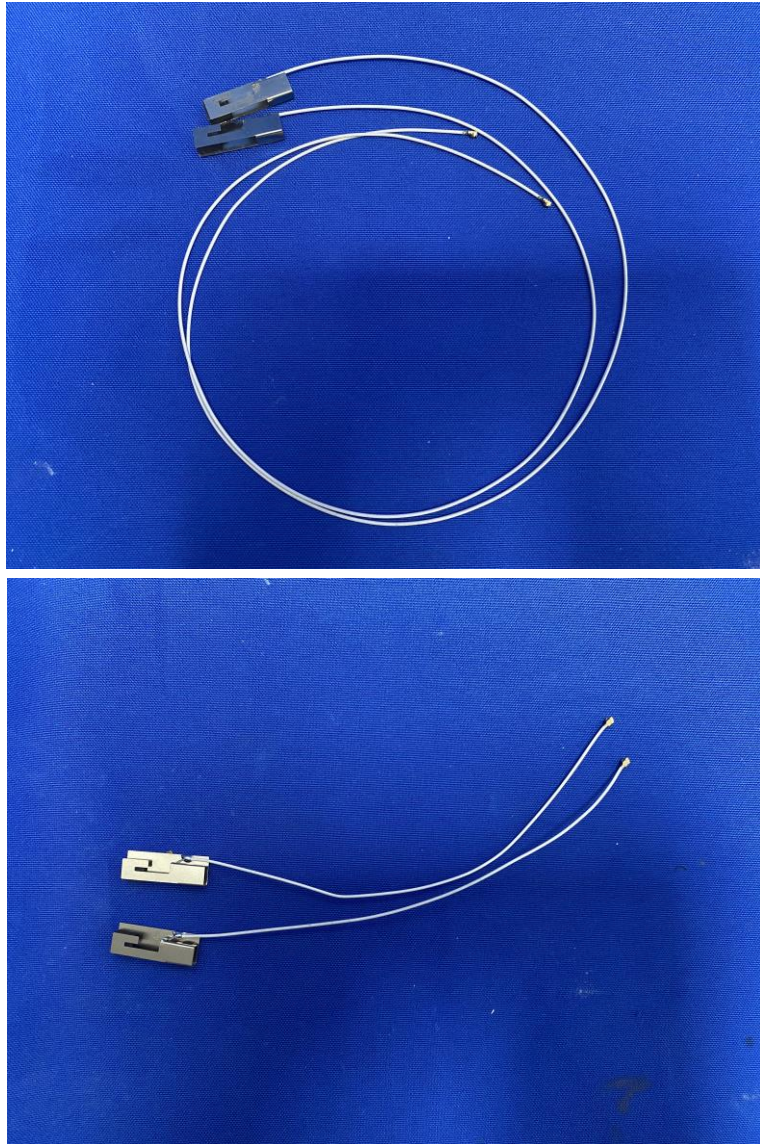
(4) EUT Photo (BT Antenna)
