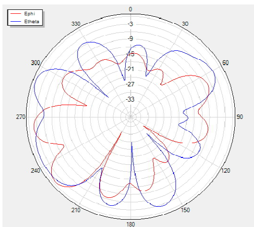
Phi=90 freq=2450MHz
