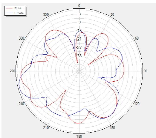
Theta=90 freq=2450MHz
