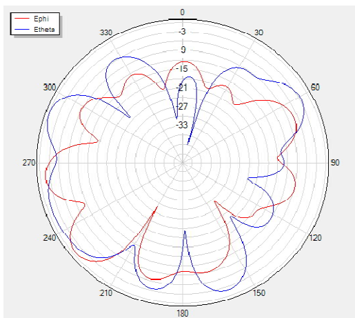
Phi=90 freq=2500MHz
