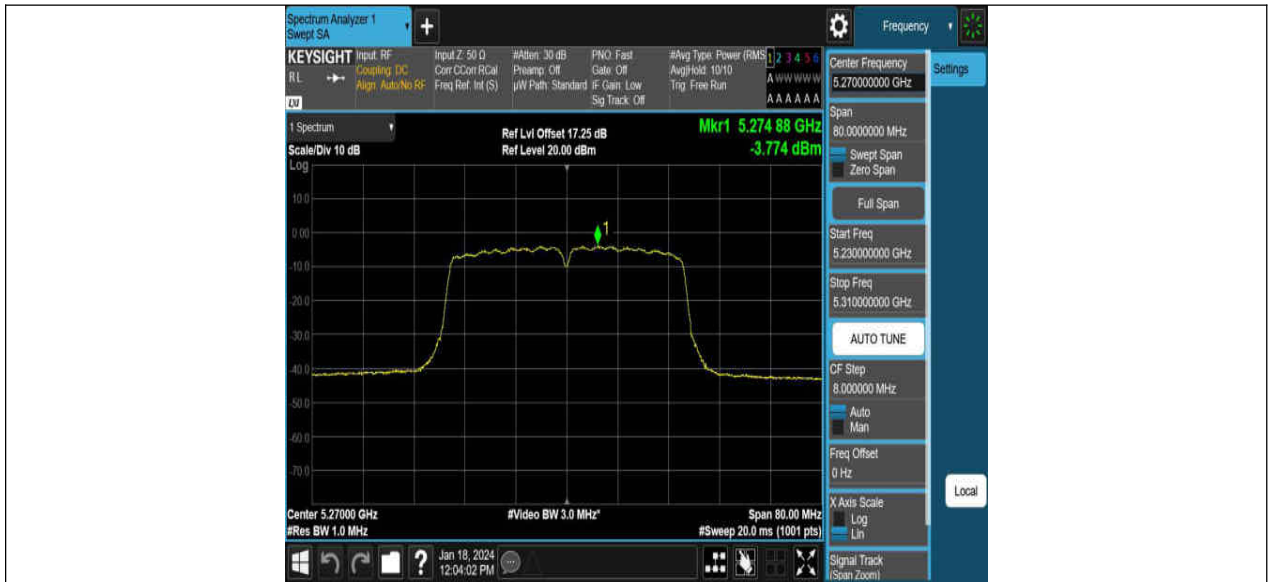
11N40MIMO Ant2 5270
