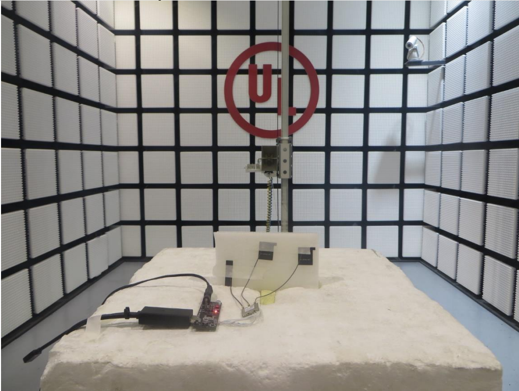
Radiated Spurious Emission Above 1 GHz – Y Axis
