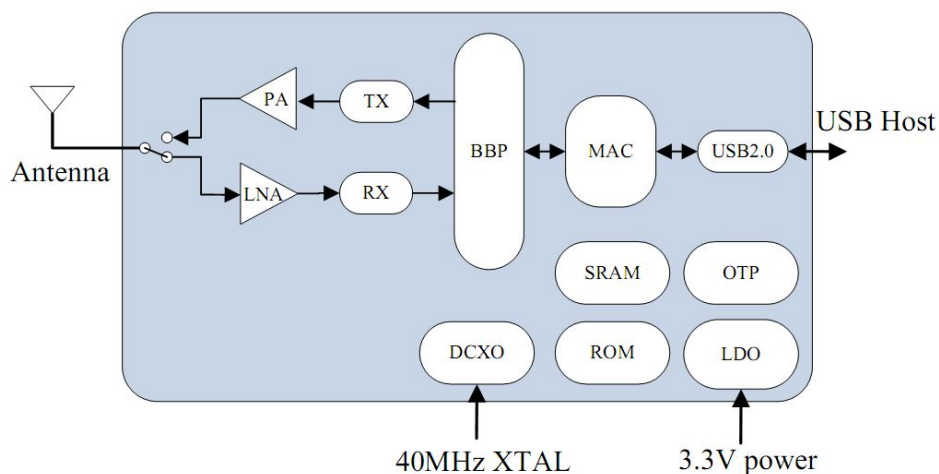
Figure 2.1 SKI.W6022.1 Block Diagram
