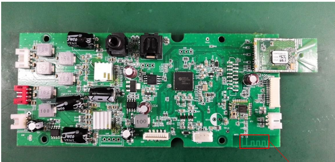
BT Antenna
