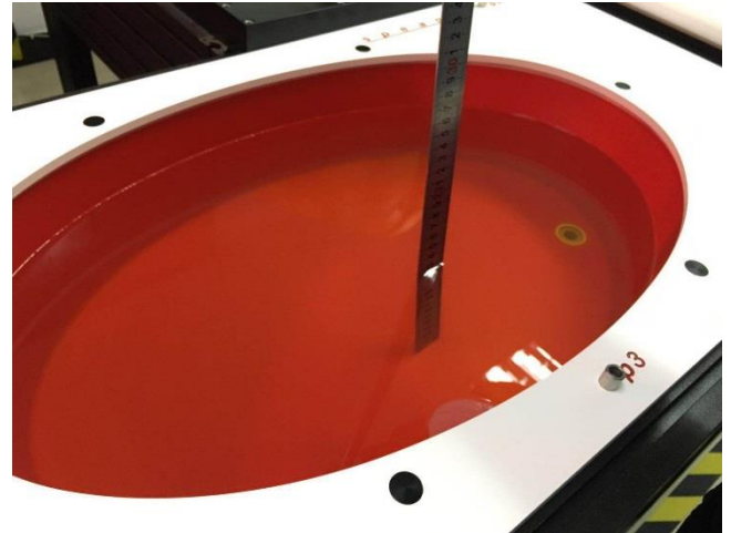
Liquid Depth in the flat phantom (16.4cm)
