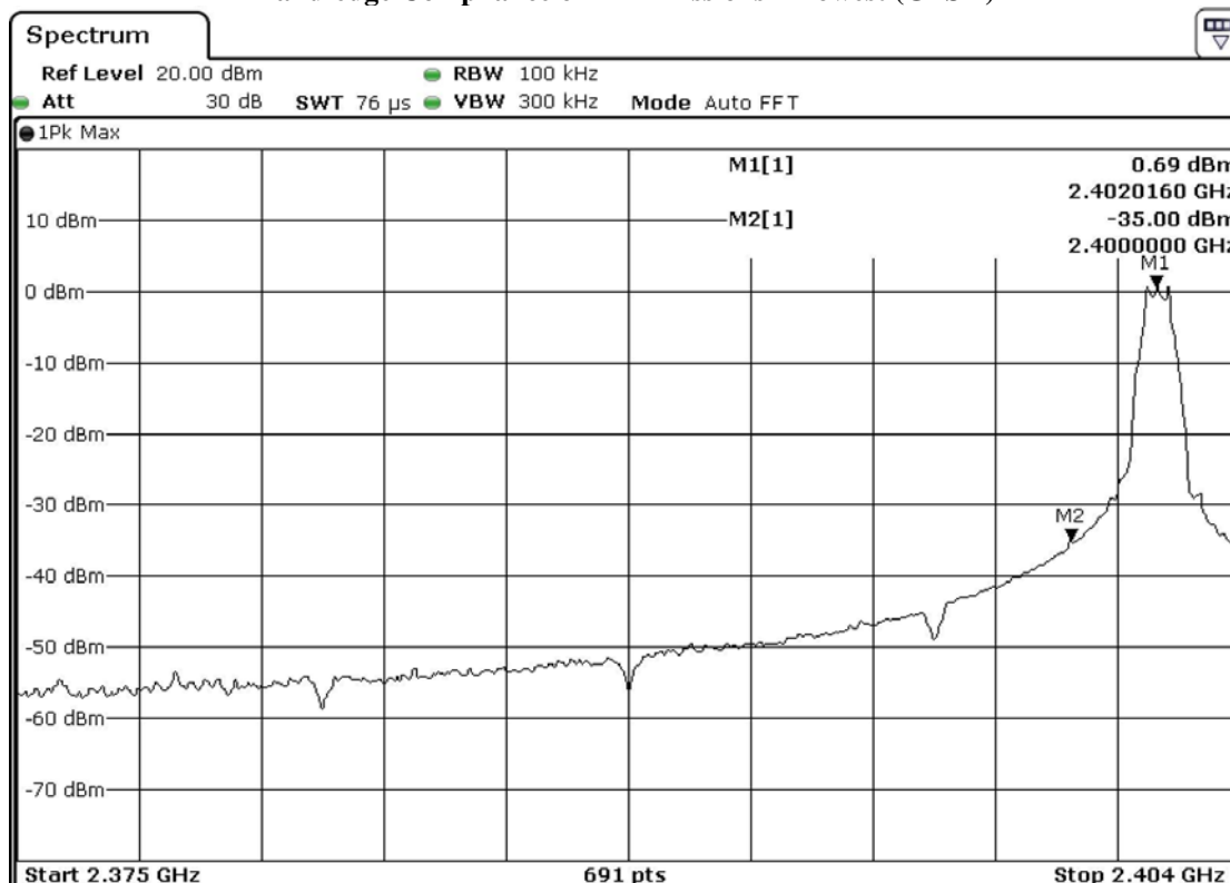
Band-edge Compliance of RF Emissions – Lowest (GFSK)
