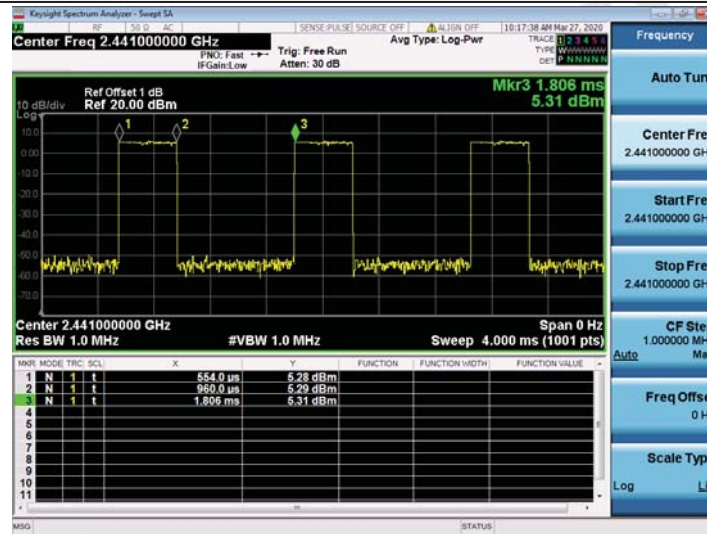
2-DH1
