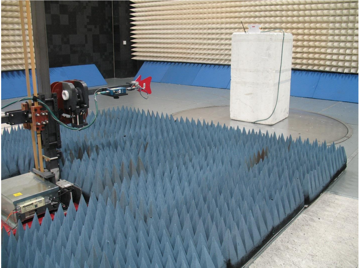
Spurious Emissions >1Ghz
