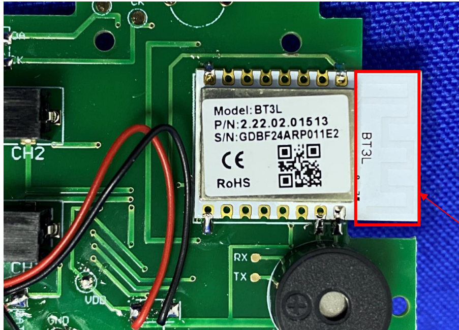
Module view
