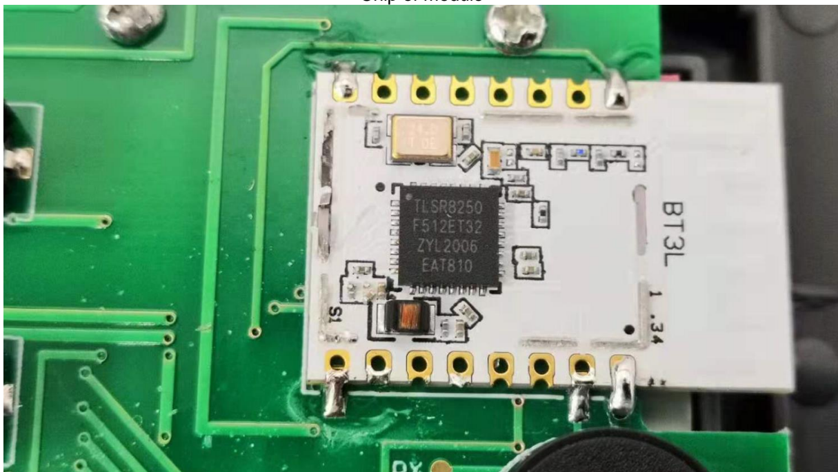
Chip of module
