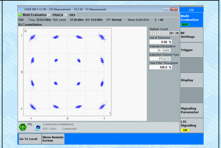
Band7-15MHz-16QAM-21100-75RB#0-PASS
