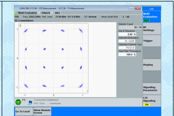
Band7-5MHz-16QAM-20775-25RB#0-PASS
