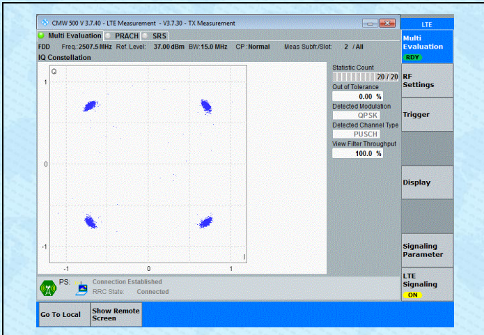
Band7-15MHz-QPSK-20825-75RB#0-PASS
