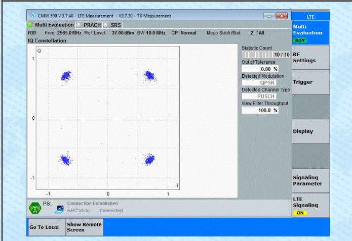
Band7-10MHz-QPSK-21400-50RB#0-PASS
