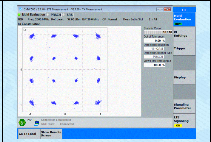
Band7-20MHz-16QAM-21350-100RB#0-PASS
