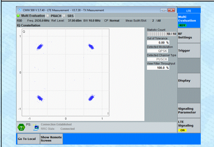
Band7-10MHz-QPSK-21100-50RB#0-PASS
