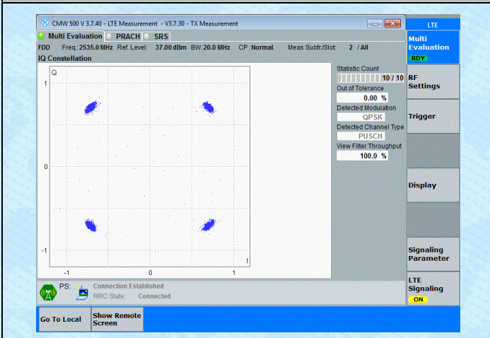
Band7-20MHz-QPSK-21100-100RB#0-PASS
