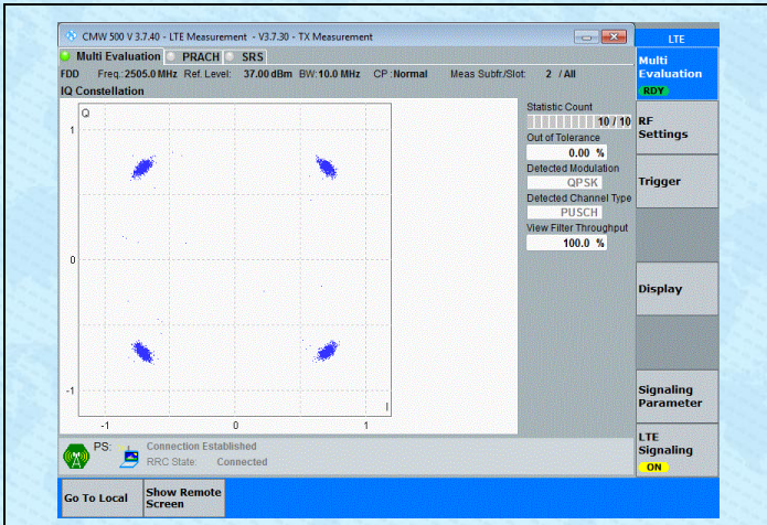
Band7-10MHz-QPSK-20800-50RB#0-PASS
