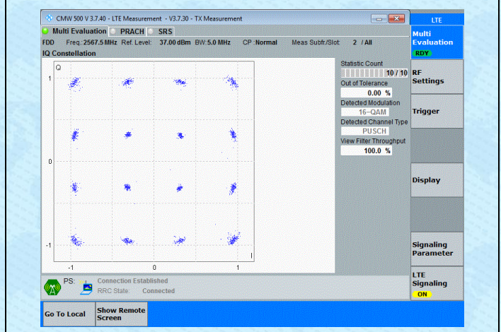
Band7-5MHz-16QAM-21425-25RB#0-PASS
