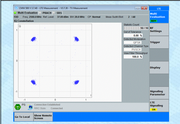
Band7-20MHz-QPSK-21350-100RB#0-PASS
