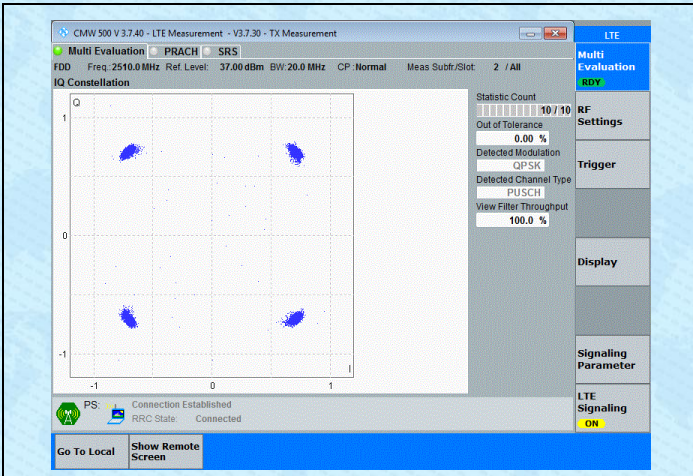
Band7-20MHz-QPSK-20850-100RB#0-PASS
