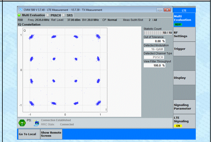
Band7-20MHz-16QAM-21100-100RB#0-PASS
