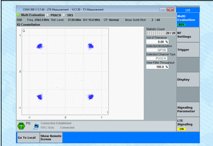
Band7-15MHz-QPSK-21375-75RB#0-PASS
