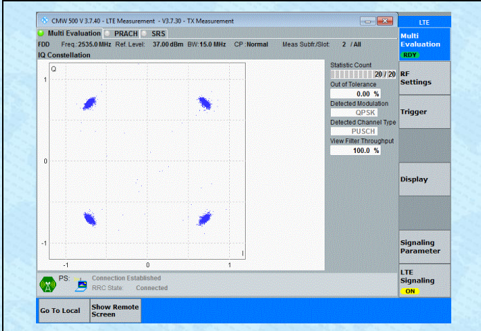
Band7-15MHz-QPSK-21100-75RB#0-PASS
