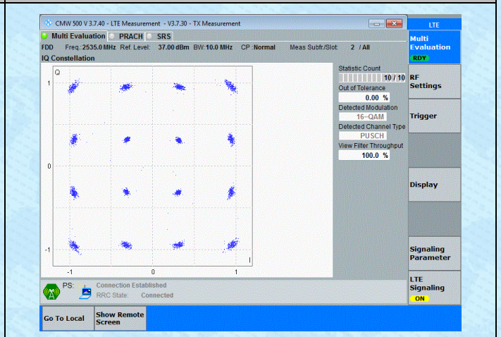
Band7-10MHz-16QAM-21100-50RB#0-PASS
