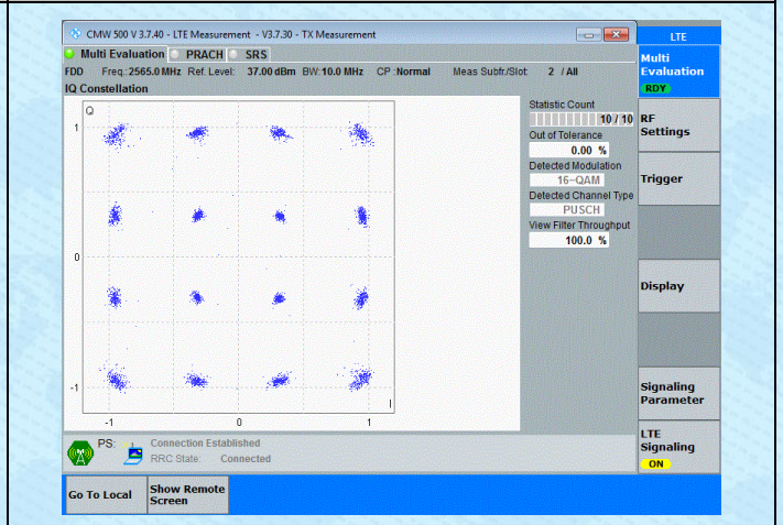
Band7-10MHz-16QAM-21400-50RB#0-PASS
