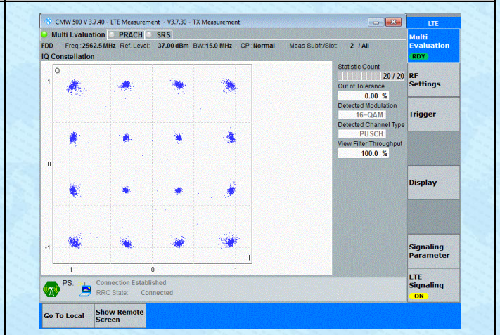
Band7-15MHz-16QAM-21375-75RB#0-PASS
