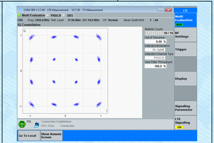
Band7-10MHz-16QAM-20800-50RB#0-PASS
