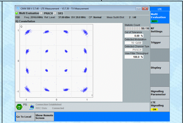
Band7-20MHz-16QAM-20850-100RB#0-PASS
