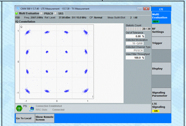
Band7-15MHz-16QAM-20825-75RB#0-PASS
