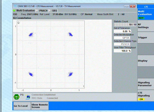
Band7-5MHz-QPSK-21425-25RB#0-PASS
