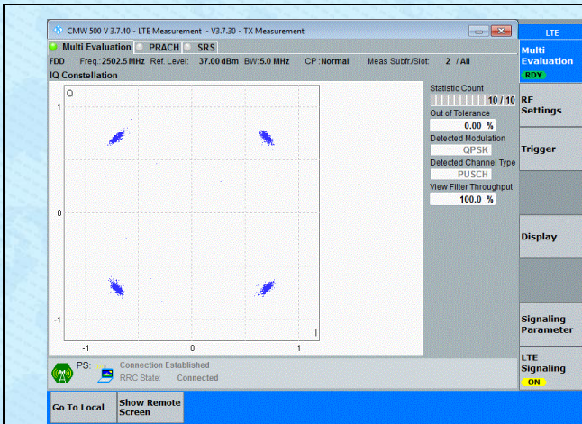
Band7-5MHz-QPSK-20775-25RB#0-PASS
