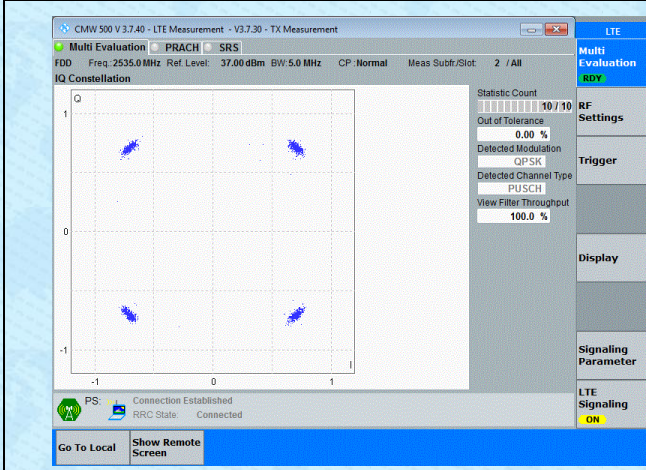
Band7-5MHz-QPSK-21100-25RB#0-PASS
