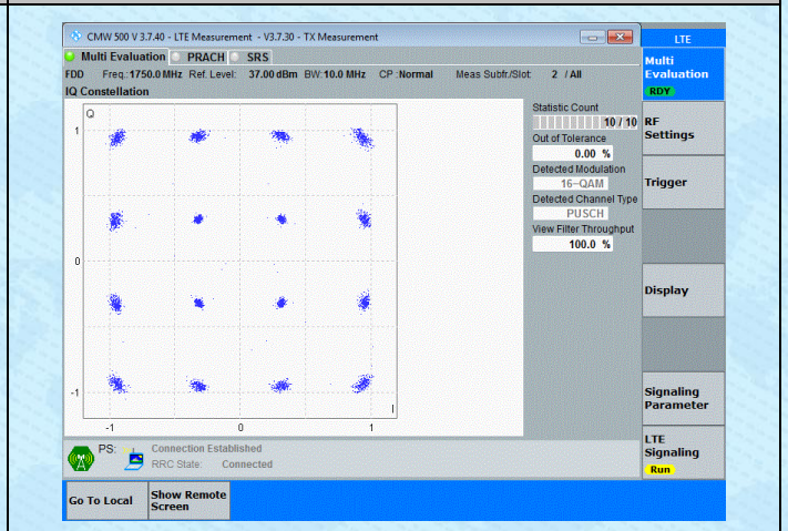
Band4-10MHz-16QAM-20350-50RB#0-PASS
