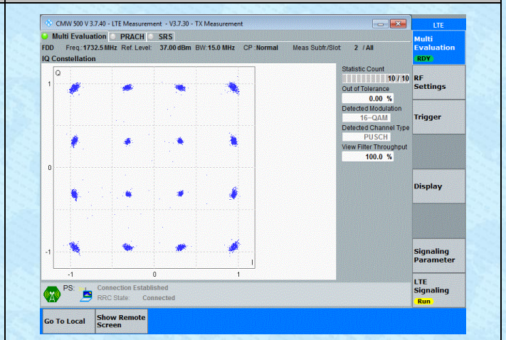
Band4-15MHz-16QAM-20175-75RB#0-PASS
