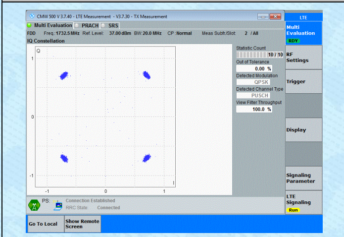
Band4-20MHz-QPSK-20175-100RB#0-PASS
