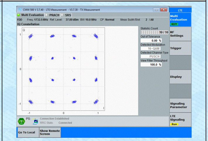
Band4-10MHz-16QAM-20175-50RB#0-PASS
