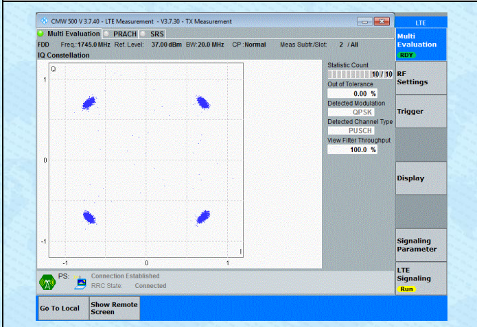
Band4-20MHz-QPSK-20300-100RB#0-PASS
