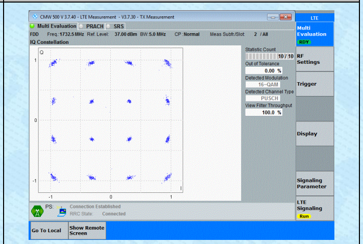
Band4-5MHz-16QAM-20175-25RB#0-PASS
