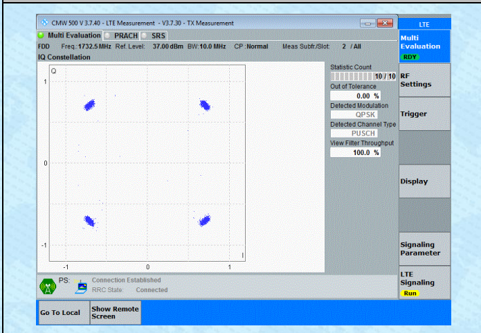
Band4-10MHz-QPSK-20175-50RB#0-PASS
