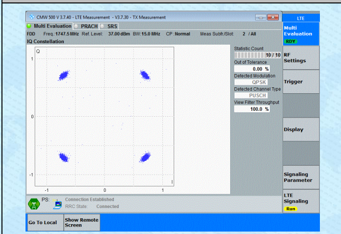
Band4-15MHz-QPSK-20325-75RB#0-PASS
