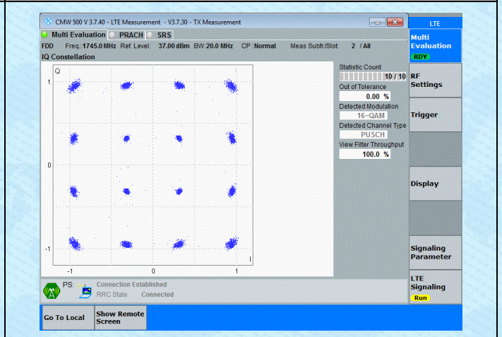
Band4-20MHz-16QAM-20300-100RB#0-PASS
