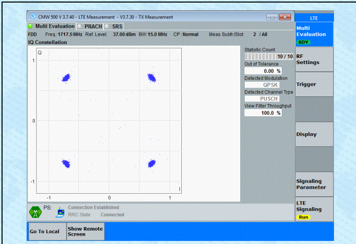
Band4-15MHz-QPSK-20025-75RB#0-PASS
