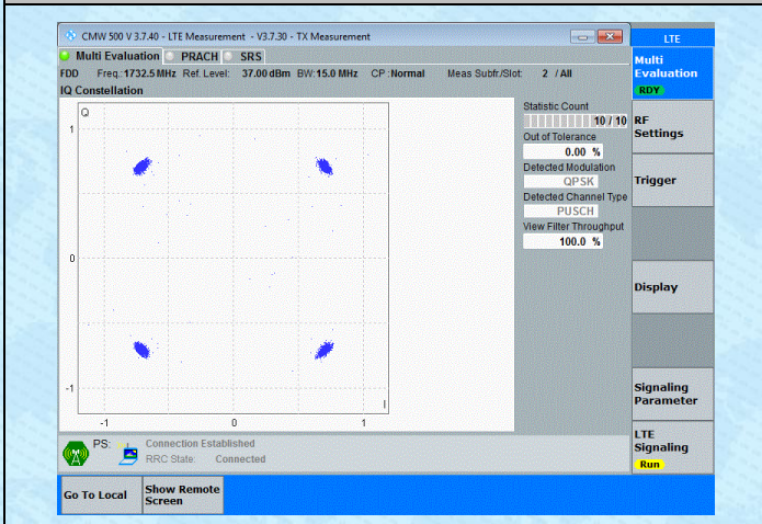
Band4-15MHz-QPSK-20175-75RB#0-PASS
