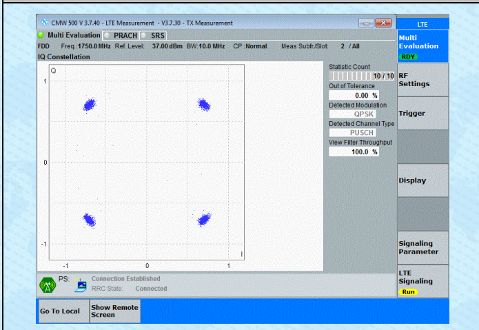
Band4-10MHz-QPSK-20350-50RB#0-PASS
