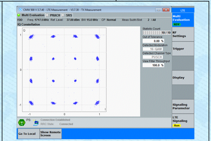
Band4-15MHz-16QAM-20025-75RB#0-PASS
