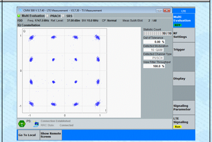
Band4-15MHz-16QAM-20325-75RB#0-PASS
