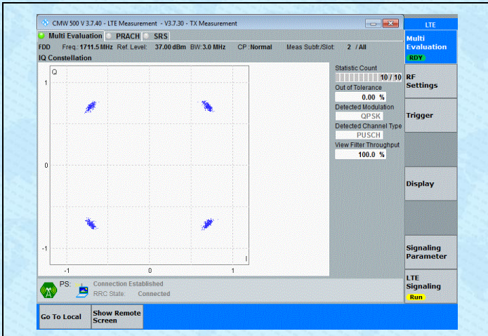
Band4-3MHz-QPSK-19965-15RB#0-PASS
