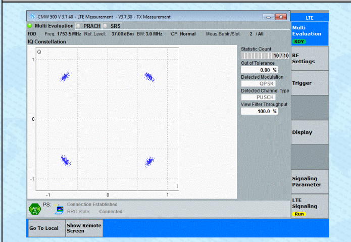
Band4-3MHz-QPSK-20385-15RB#0-PASS
