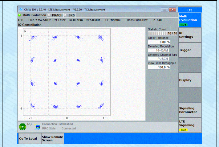
Band4-5MHz-16QAM-20375-25RB#0-PASS
