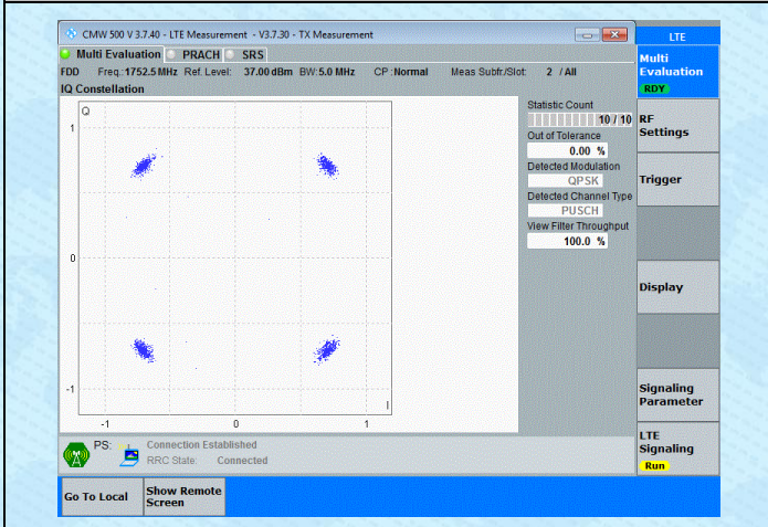
Band4-5MHz-QPSK-20375-25RB#0-PASS
