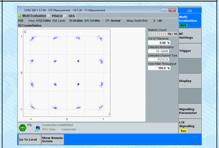
Band4-3MHz-16QAM-20385-15RB#0-PASS
