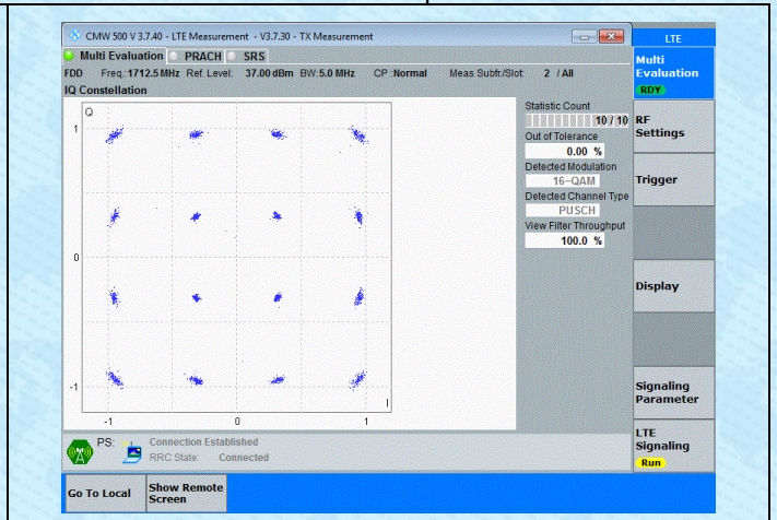
Band4-5MHz-16QAM-19975-25RB#0-PASS
