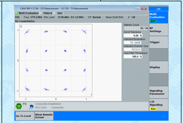
Band4-3MHz-16QAM-19965-15RB#0-PASS
