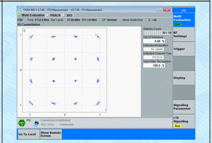
Band4-3MHz-16QAM-20175-15RB#0-PASS
