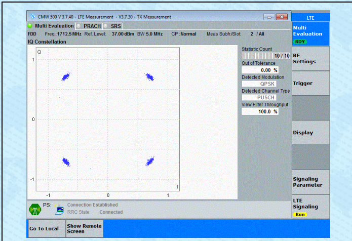
Band4-5MHz-QPSK-19975-25RB#0-PASS
