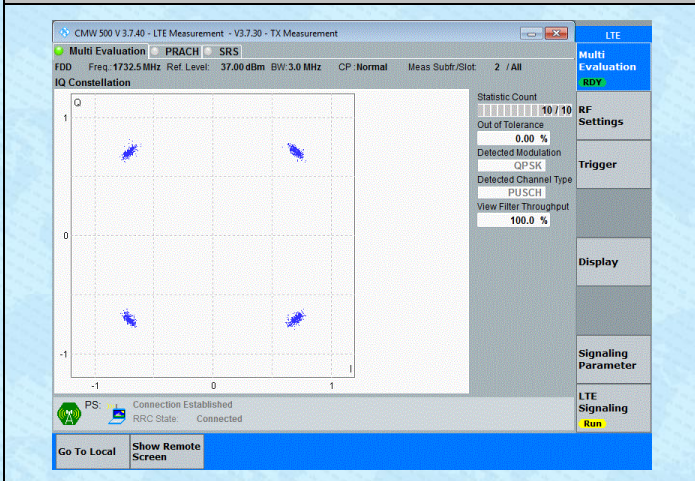
Band4-3MHz-QPSK-20175-15RB#0-PASS
