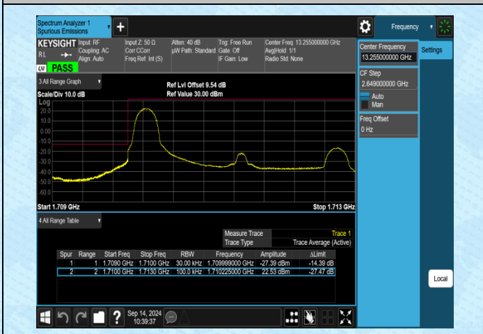
Band4-3MHz-QPSK-19965-1RB#0-PASS
