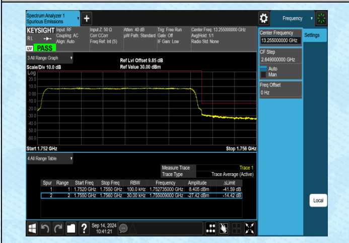
Band4-3MHz-16QAM-20385-15RB#0-PASS
