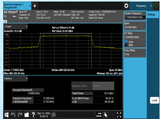
Band4-10MHz-16QAM-20350-50RB#0-PASS
