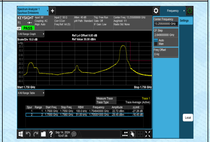
Band4-5MHz-QPSK-20375-1RB#24-PASS
