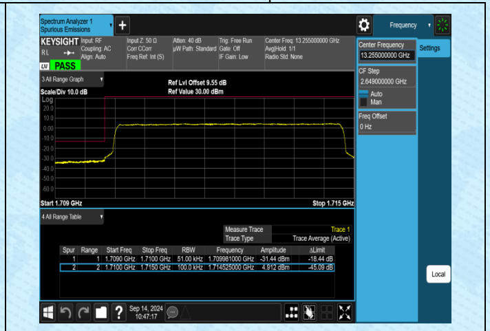
Band4-5MHz-16QAM-19975-25RB#0-PASS
