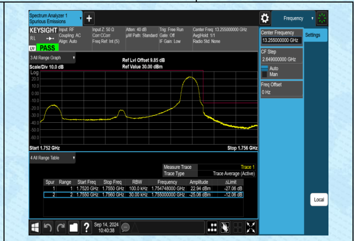
Band4-3MHz-QPSK-20385-1RB#14-PASS
