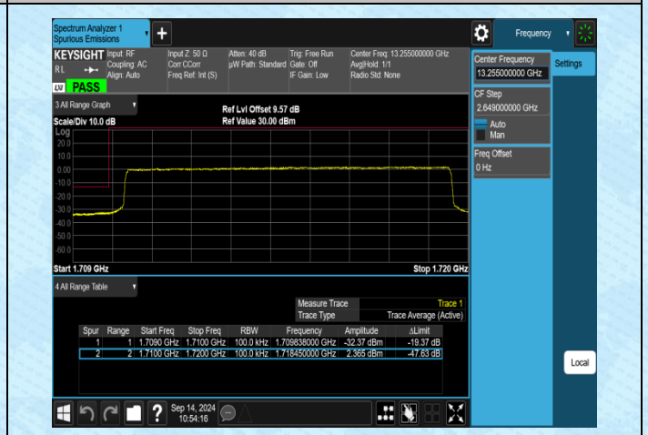
Band4-10MHz-16QAM-20000-50RB#0-PASS
