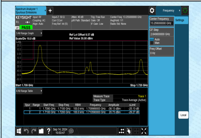
Band4-10MHz-16QAM-20000-1RB#0-PASS
