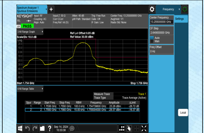
Band4-1.4MHz-QPSK-20393-1RB#5-PASS
