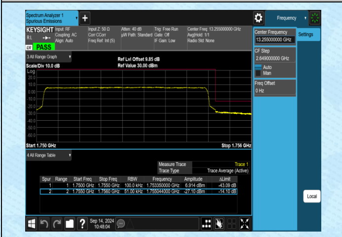
Band4-5MHz-QPSK-20375-25RB#0-PASS
