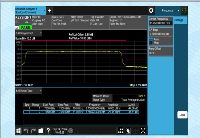
Band4-5MHz-16QAM-20375-25RB#0-PASS
