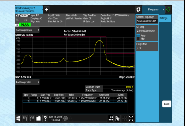
Band4-3MHz-16QAM-20385-1RB#14-PASS
