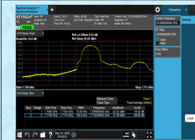
Band4-1.4MHz-16QAM-19957-1RB#0-PASS
