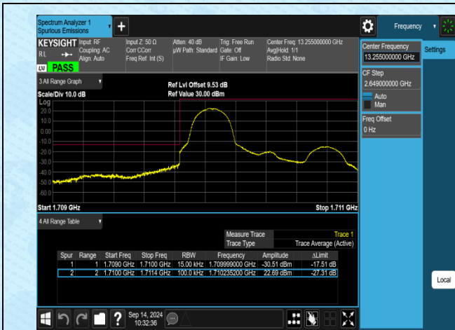
Band4-1.4MHz-QPSK-19957-1RB#0-PASS
