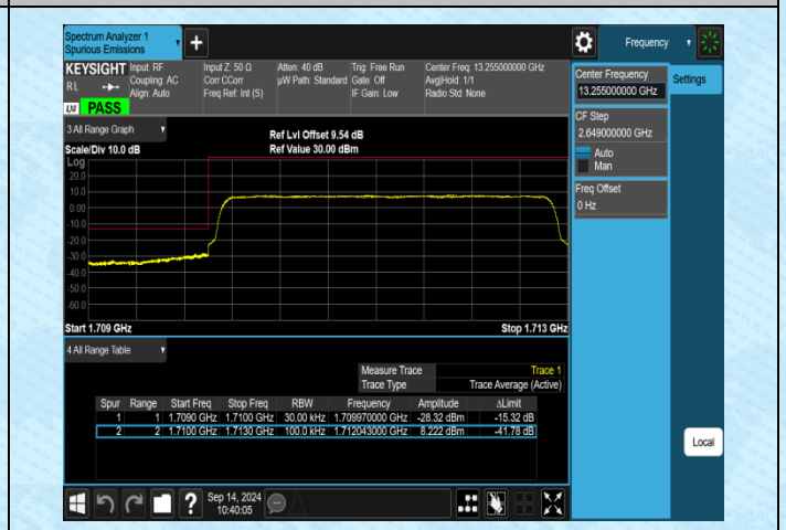
Band4-3MHz-QPSK-19965-15RB#0-PASS
