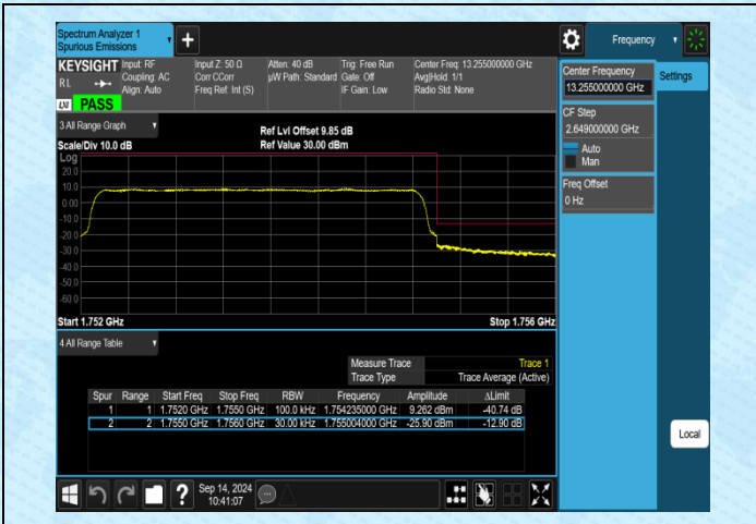
Band4-3MHz-QPSK-20385-15RB#0-PASS
