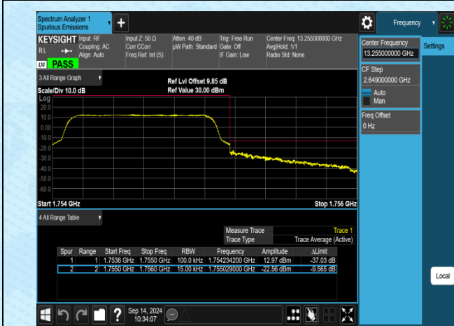
Band4-1.4MHz-QPSK-20393-6RB#0-PASS
