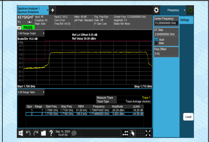
Band4-5MHz-QPSK-19975-25RB#0-PASS
