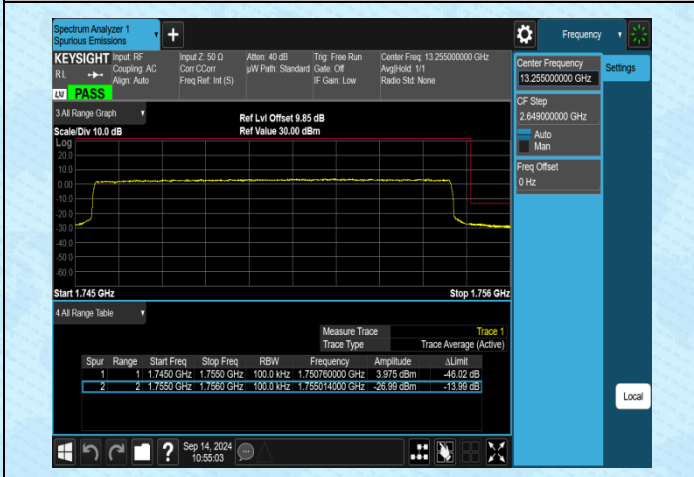
Band4-10MHz-QPSK-20350-50RB#0-PASS
