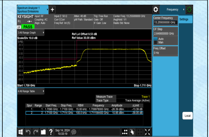
Band4-1.4MHz-16QAM-19957-6RB#0-PASS
