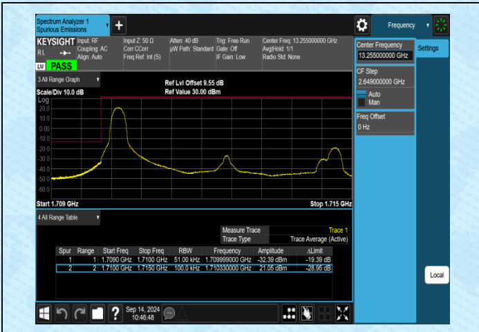
Band4-5MHz-16QAM-19975-1RB#0-PASS
