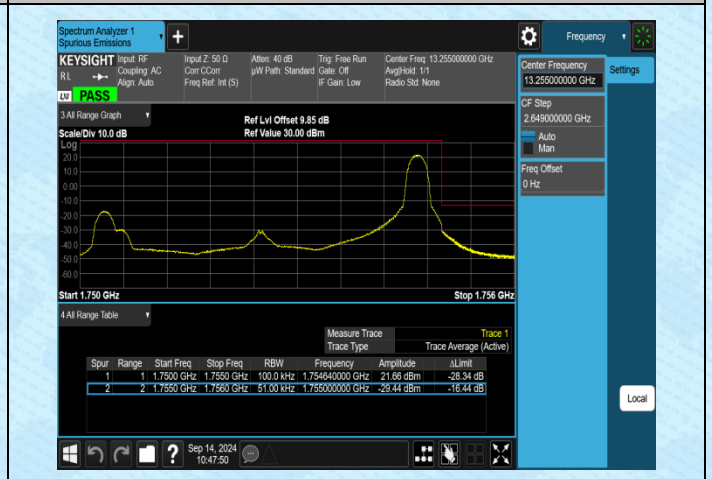
Band4-5MHz-16QAM-20375-1RB#24-PASS
