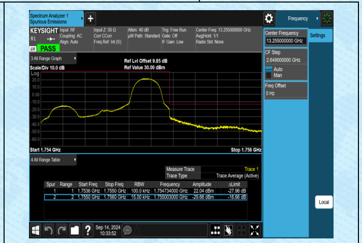
Band4-1.4MHz-16QAM-20393-1RB#5-PASS
