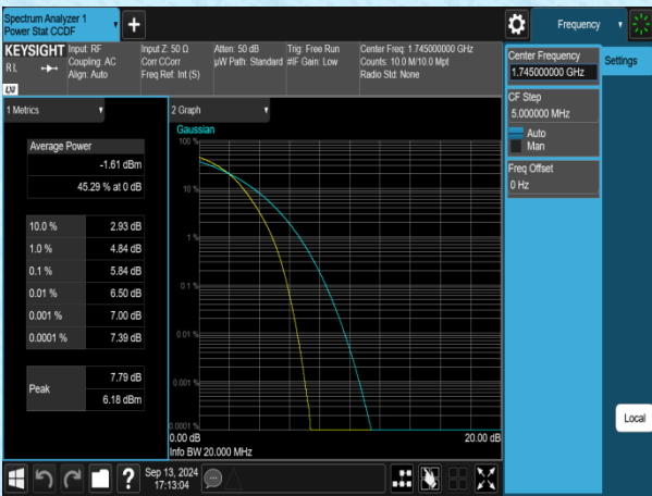
Band4-20MHz-16QAM-20300-1RB#0-PASS
