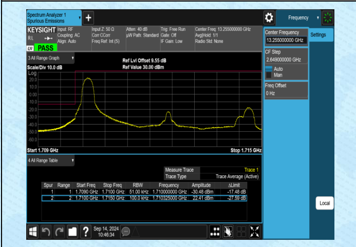
Band4-5MHz-QPSK-19975-1RB#0-PASS
