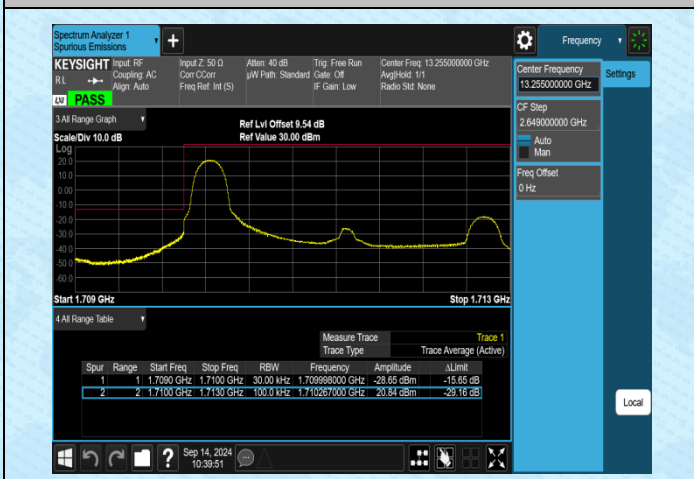
Band4-3MHz-16QAM-19965-1RB#0-PASS
